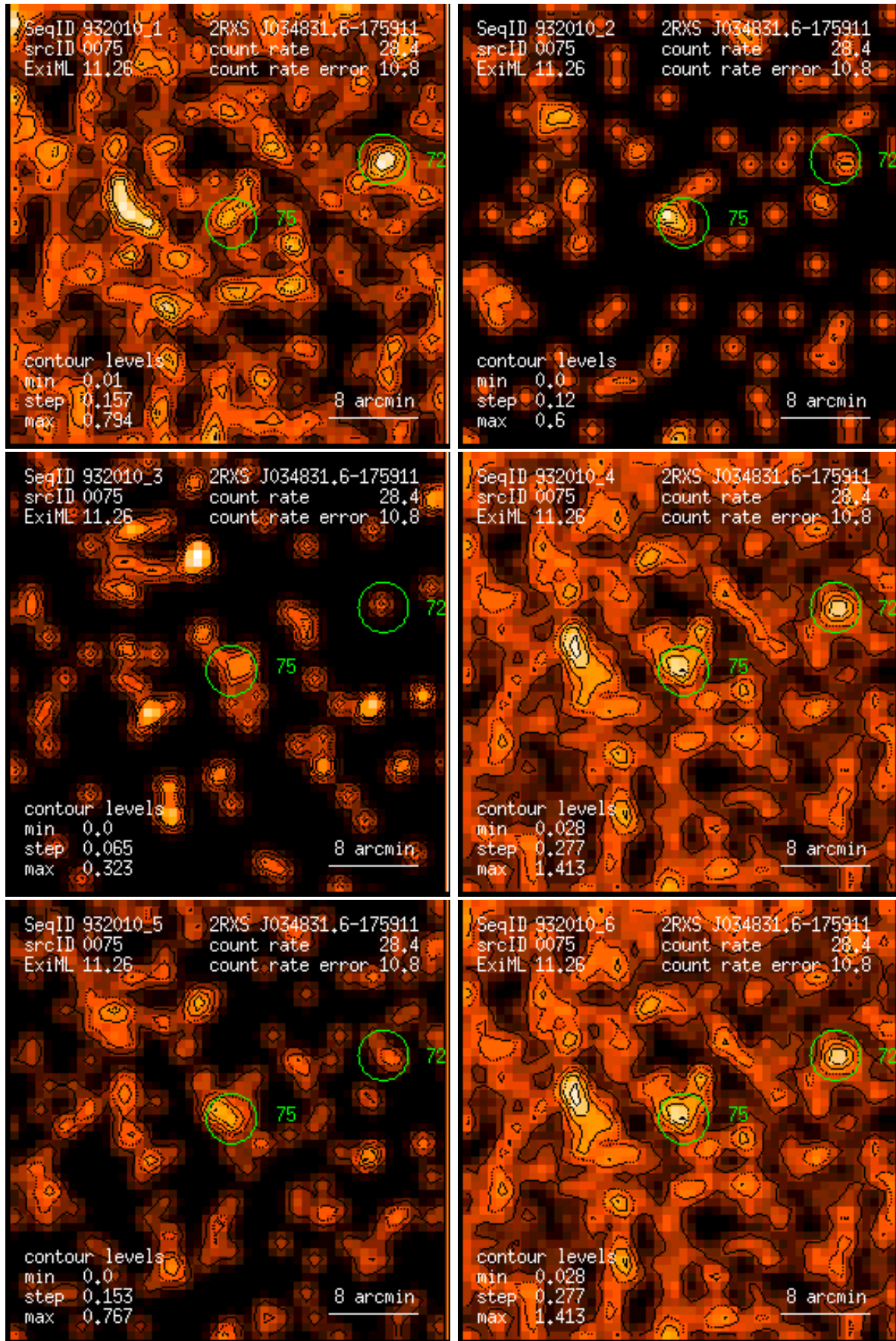
Figure 75: RASS 932010: detection 0075: band rate images, Gaussian filter: (1) PSPC channels 11 – 41, (2) 52 – 90, (3) 91 – 201, (4) 11 – 235, (5) 52 – 201, (6) 11 – 201. Broad band rates in counts/ks. Band rate contour levels in counts/ks/arcmin 2 .
