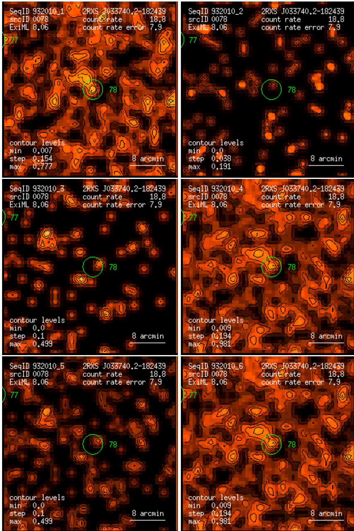
Figure 78: RASS 932010: detection 0078: band rate images, Gaussian filter: (1) PSPC channels 11 – 41, (2) 52 – 90, (3) 91 – 201, (4) 11 – 235, (5) 52 – 201, (6) 11 – 201. Broad band rates in counts/ks. Band rate contour levels in counts/ks/arcmin 2 .
