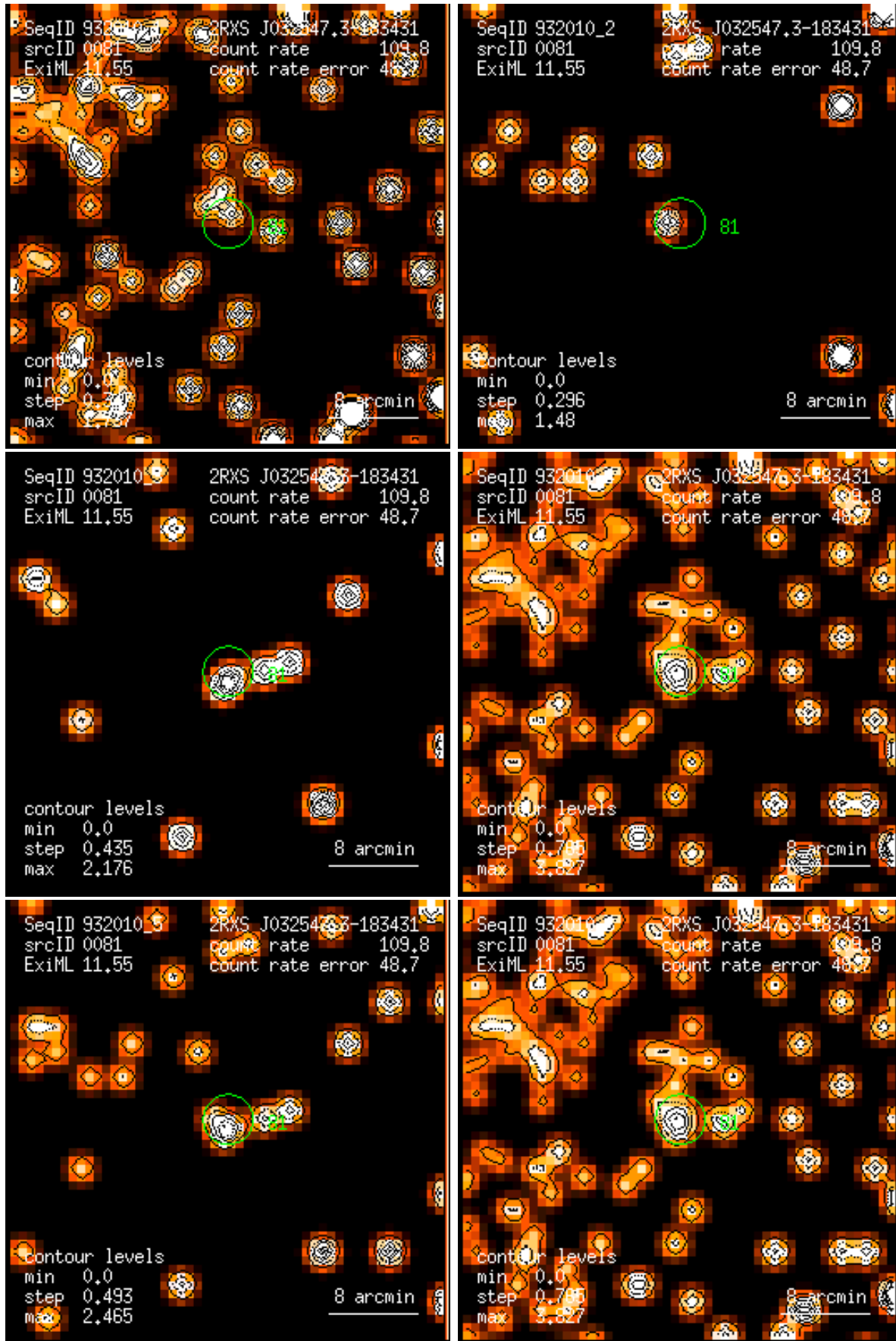
Figure 81: RASS 932010: detection 0081: band rate images, Gaussian filter: (1) PSPC channels 11 – 41, (2) 52 – 90, (3) 91 – 201, (4) 11 – 235, (5) 52 – 201, (6) 11 – 201. Broad band rates in counts/ks. Band rate contour levels in counts/ks/arcmin 2 .
