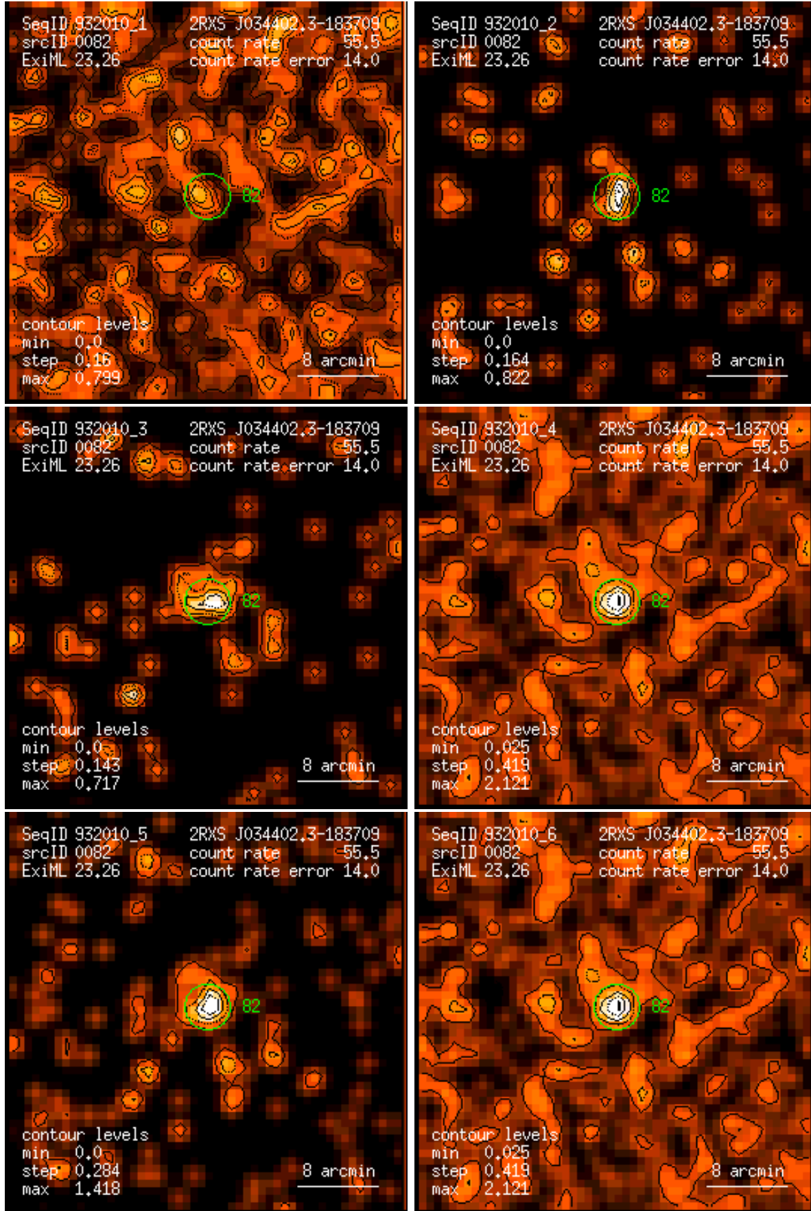
Figure 82: RASS 932010: detection 0082: band rate images, Gaussian filter: (1) PSPC channels 11 – 41, (2) 52 – 90, (3) 91 – 201, (4) 11 – 235, (5) 52 – 201, (6) 11 – 201. Broad band rates in counts/ks. Band rate contour levels in counts/ks/arcmin 2 .
