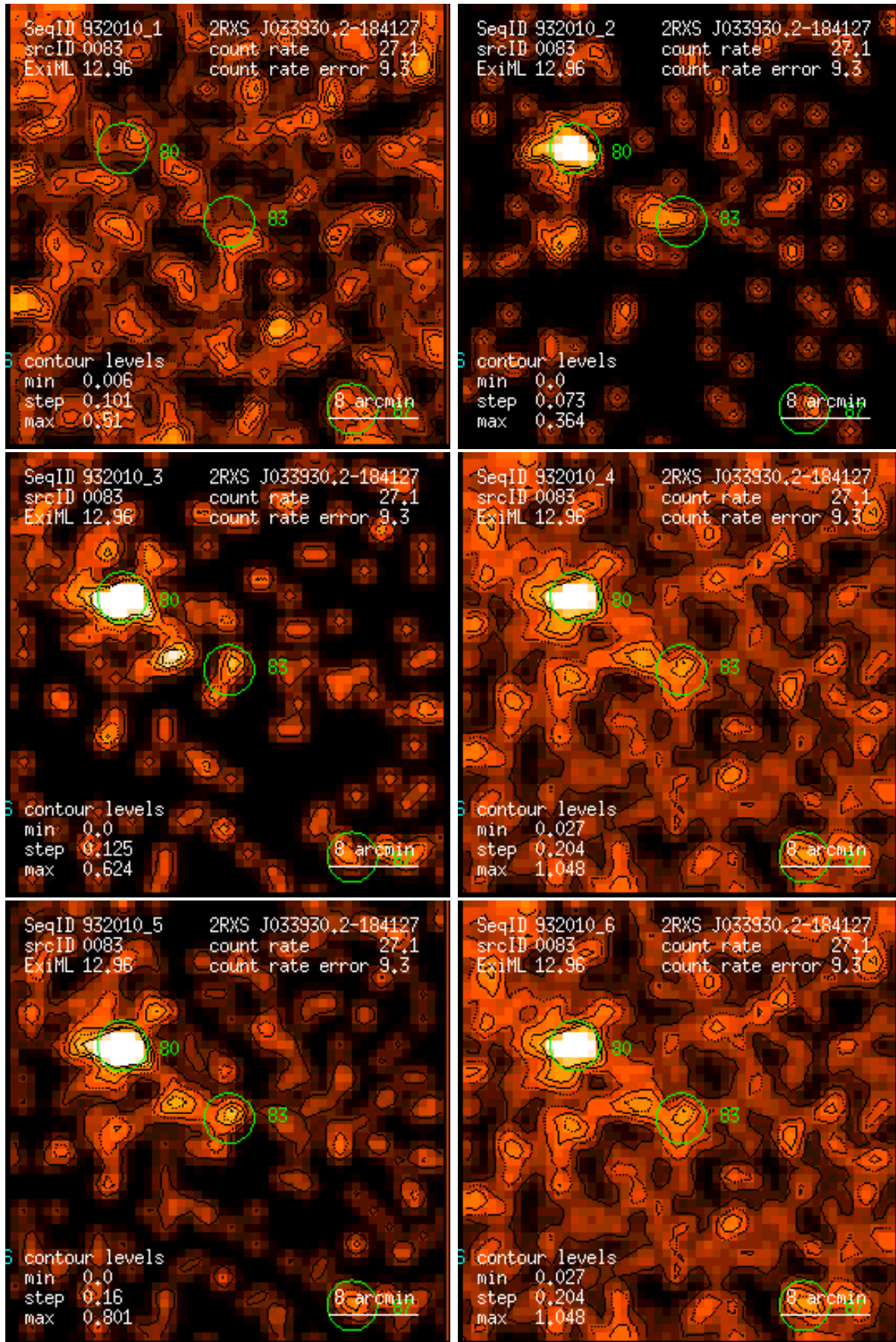
Figure 83: RASS 932010: detection 0083: band rate images, Gaussian filter: (1) PSPC channels 11 – 41, (2) 52 – 90, (3) 91 – 201, (4) 11 – 235, (5) 52 – 201, (6) 11 – 201. Broad band rates in counts/ks. Band rate contour levels in counts/ks/arcmin 2 .
