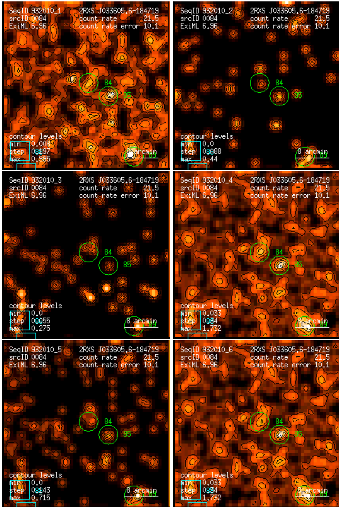
Figure 84: RASS 932010: detection 0084: band rate images, Gaussian filter: (1) PSPC channels 11 – 41, (2) 52 – 90, (3) 91 – 201, (4) 11 – 235, (5) 52 – 201, (6) 11 – 201. Broad band rates in counts/ks. Band rate contour levels in counts/ks/arcmin 2 .
