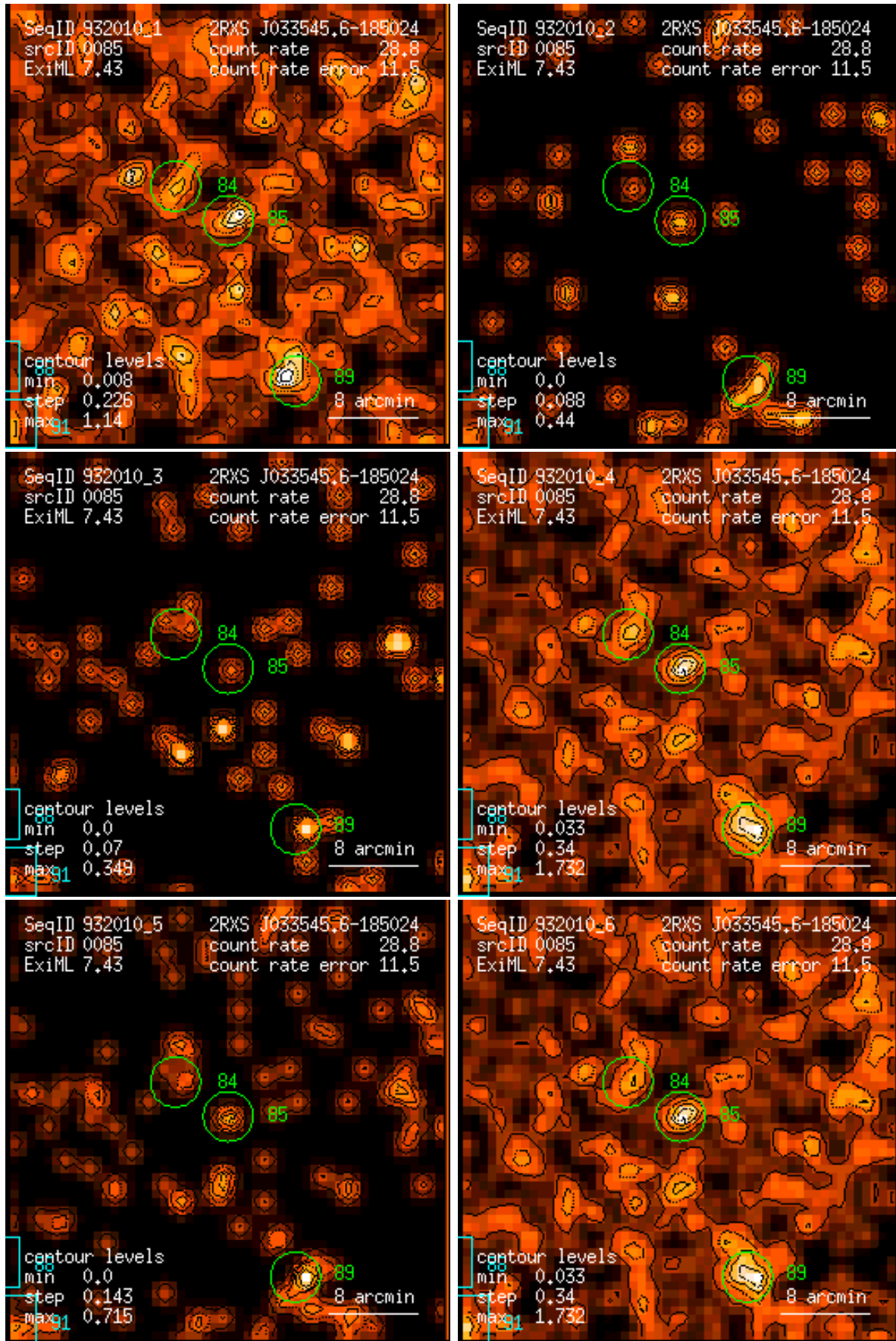
Figure 85: RASS 932010: detection 0085: band rate images, Gaussian filter: (1) PSPC channels 11 – 41, (2) 52 – 90, (3) 91 – 201, (4) 11 – 235, (5) 52 – 201, (6) 11 – 201. Broad band rates in counts/ks. Band rate contour levels in counts/ks/arcmin 2 .
