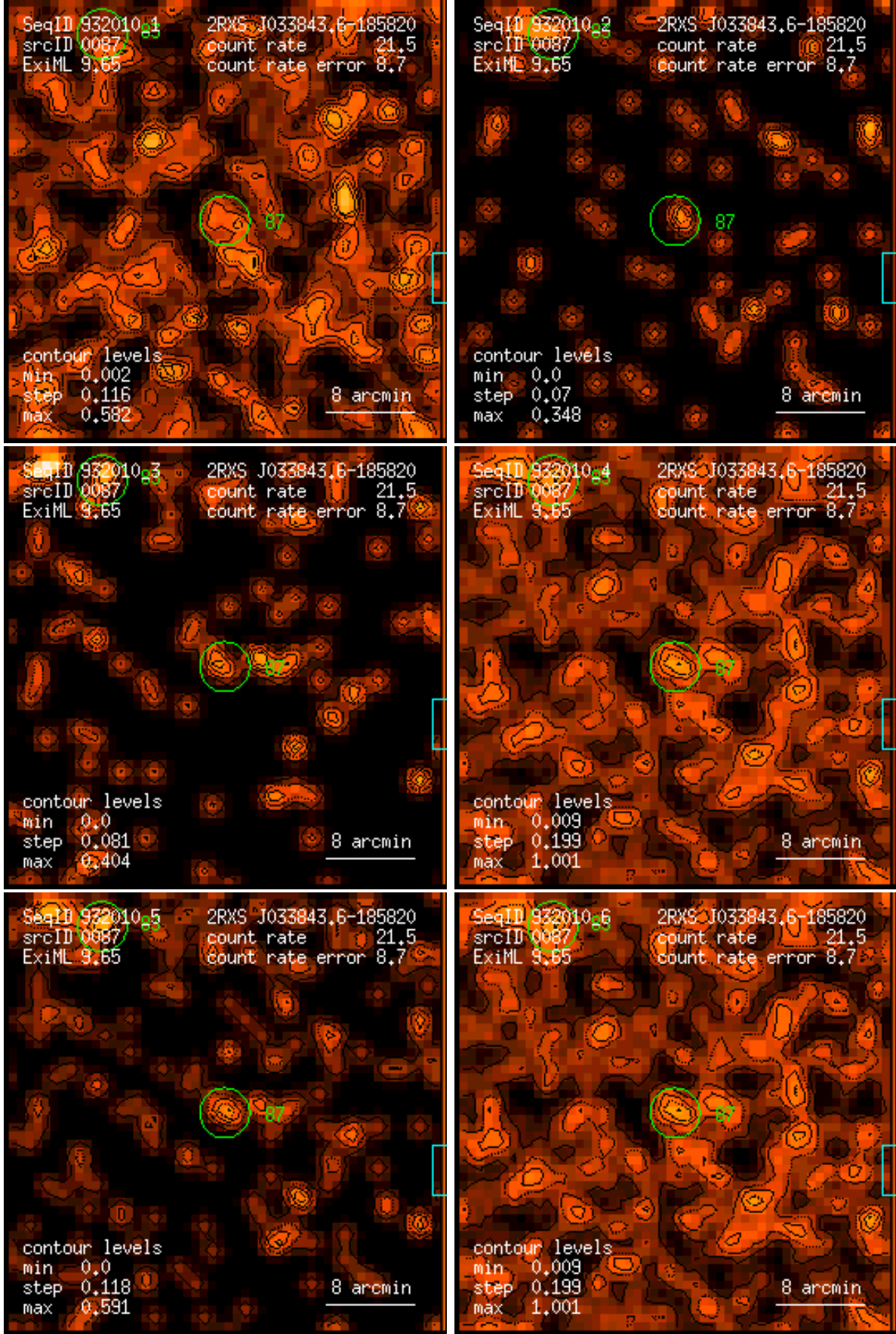
Figure 87: RASS 932010: detection 0087: band rate images, Gaussian filter: (1) PSPC channels 11 – 41, (2) 52 – 90, (3) 91 – 201, (4) 11 – 235, (5) 52 – 201, (6) 11 – 201. Broad band rates in counts/ks. Band rate contour levels in counts/ks/arcmin 2 .
