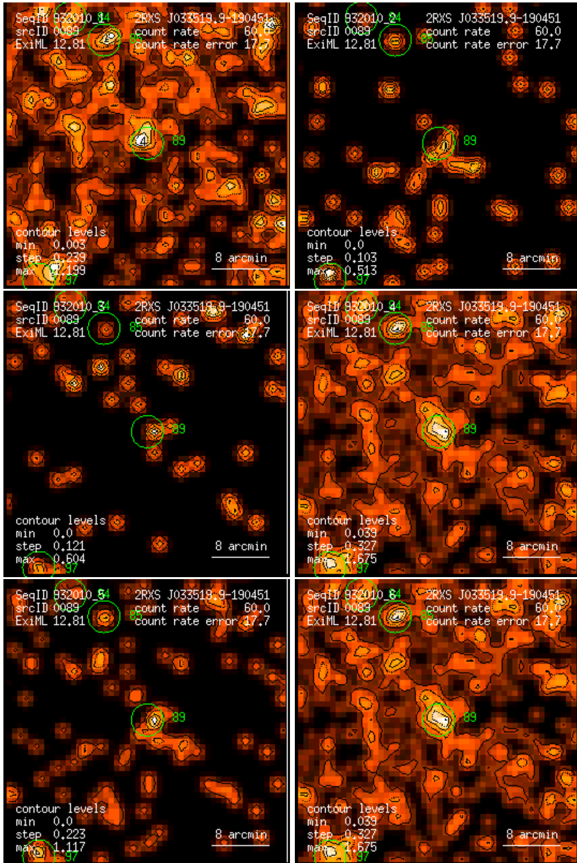
Figure 89: RASS 932010: detection 0089: band rate images, Gaussian filter: (1) PSPC channels 11 – 41, (2) 52 – 90, (3) 91 – 201, (4) 11 – 235, (5) 52 – 201, (6) 11 – 201. Broad band rates in counts/ks. Band rate contour levels in counts/ks/arcmin 2 .
