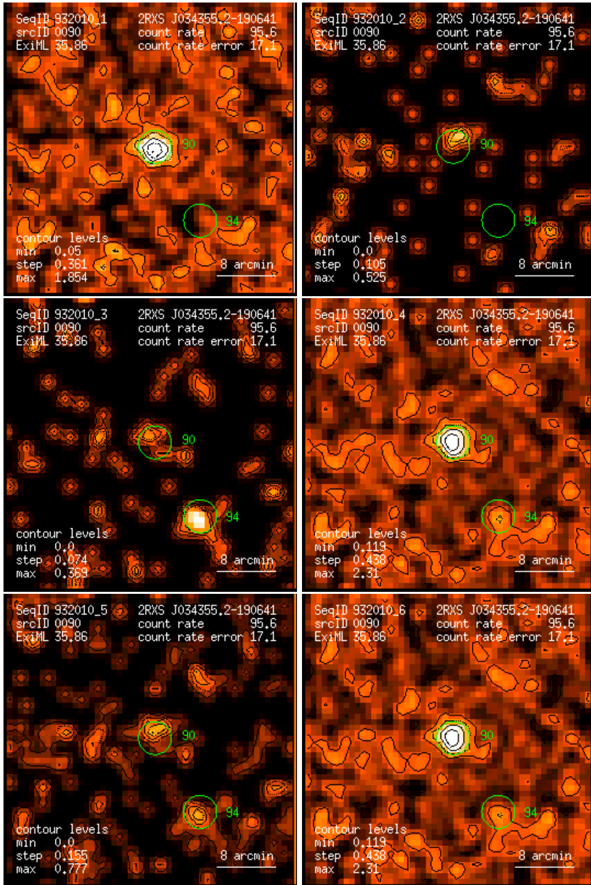
Figure 90: RASS 932010: detection 0090: band rate images, Gaussian filter: (1) PSPC channels 11 – 41, (2) 52 – 90, (3) 91 – 201, (4) 11 – 235, (5) 52 – 201, (6) 11 – 201. Broad band rates in counts/ks. Band rate contour levels in counts/ks/arcmin 2 .
