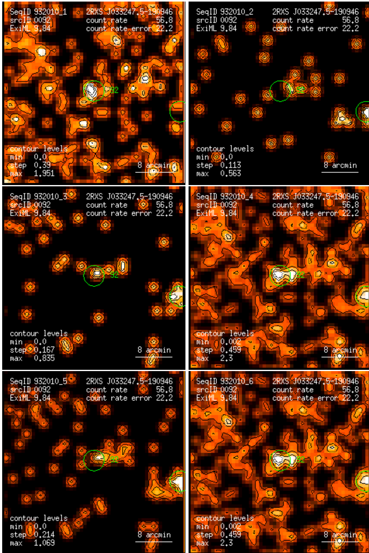
Figure 92: RASS 932010: detection 0092: band rate images, Gaussian filter: (1) PSPC channels 11 – 41, (2) 52 – 90, (3) 91 – 201, (4) 11 – 235, (5) 52 – 201, (6) 11 – 201. Broad band rates in counts/ks. Band rate contour levels in counts/ks/arcmin 2 .
