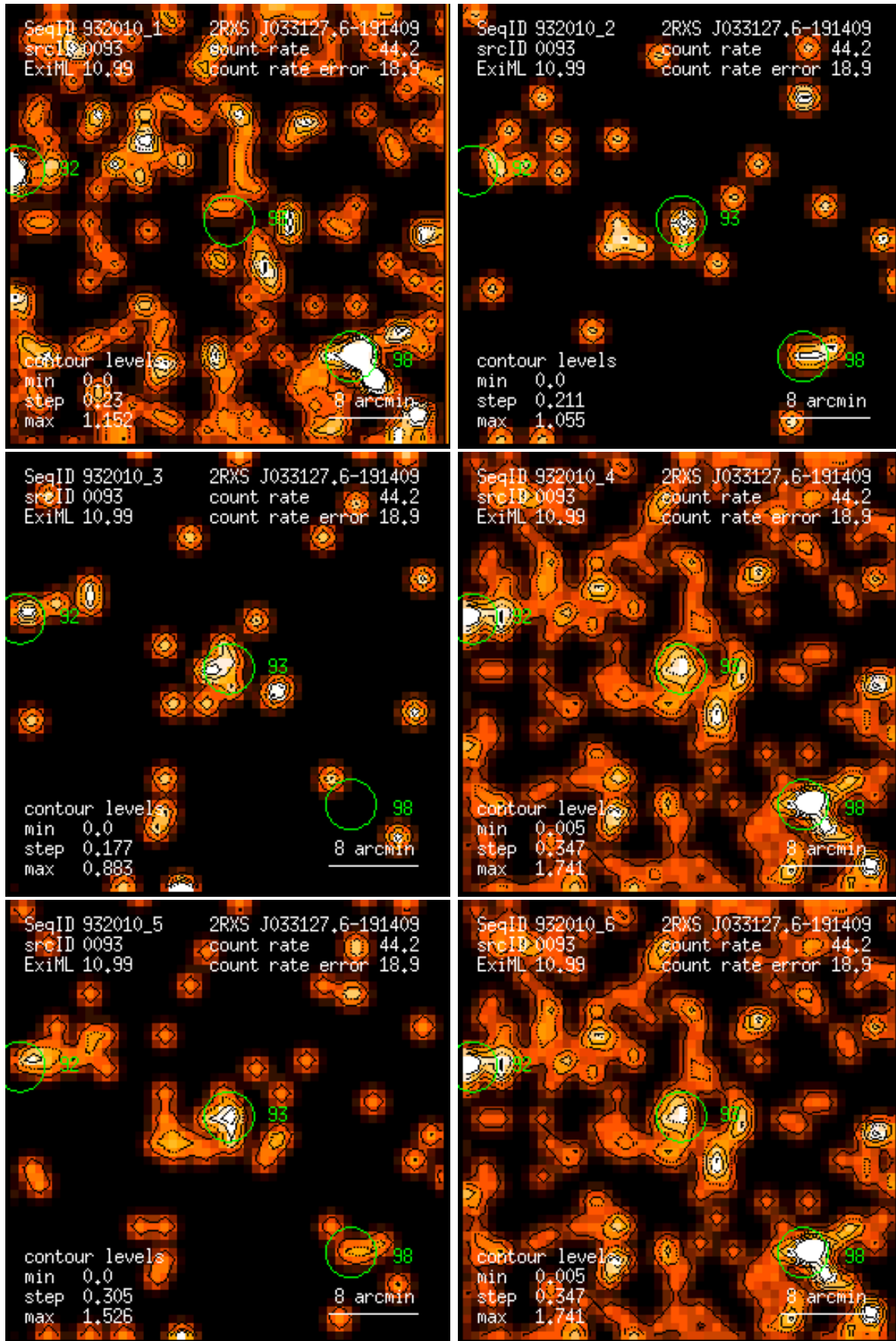
Figure 93: RASS 932010: detection 0093: band rate images, Gaussian filter: (1) PSPC channels 11 – 41, (2) 52 – 90, (3) 91 – 201, (4) 11 – 235, (5) 52 – 201, (6) 11 – 201. Broad band rates in counts/ks. Band rate contour levels in counts/ks/arcmin 2 .
