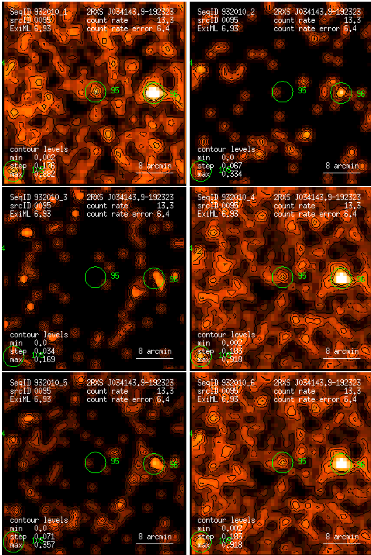
Figure 95: RASS 932010: detection 0095: band rate images, Gaussian filter: (1) PSPC channels 11 – 41, (2) 52 – 90, (3) 91 – 201, (4) 11 – 235, (5) 52 – 201, (6) 11 – 201. Broad band rates in counts/ks. Band rate contour levels in counts/ks/arcmin 2 .
