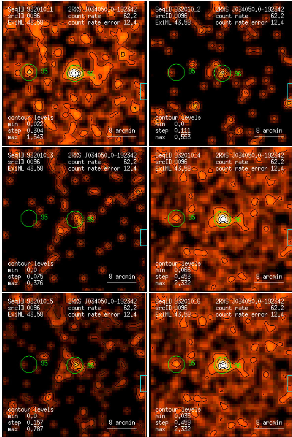
Figure 96: RASS 932010: detection 0096: band rate images, Gaussian filter: (1) PSPC channels 11 – 41, (2) 52 – 90, (3) 91 – 201, (4) 11 – 235, (5) 52 – 201, (6) 11 – 201. Broad band rates in counts/ks. Band rate contour levels in counts/ks/arcmin 2 .
