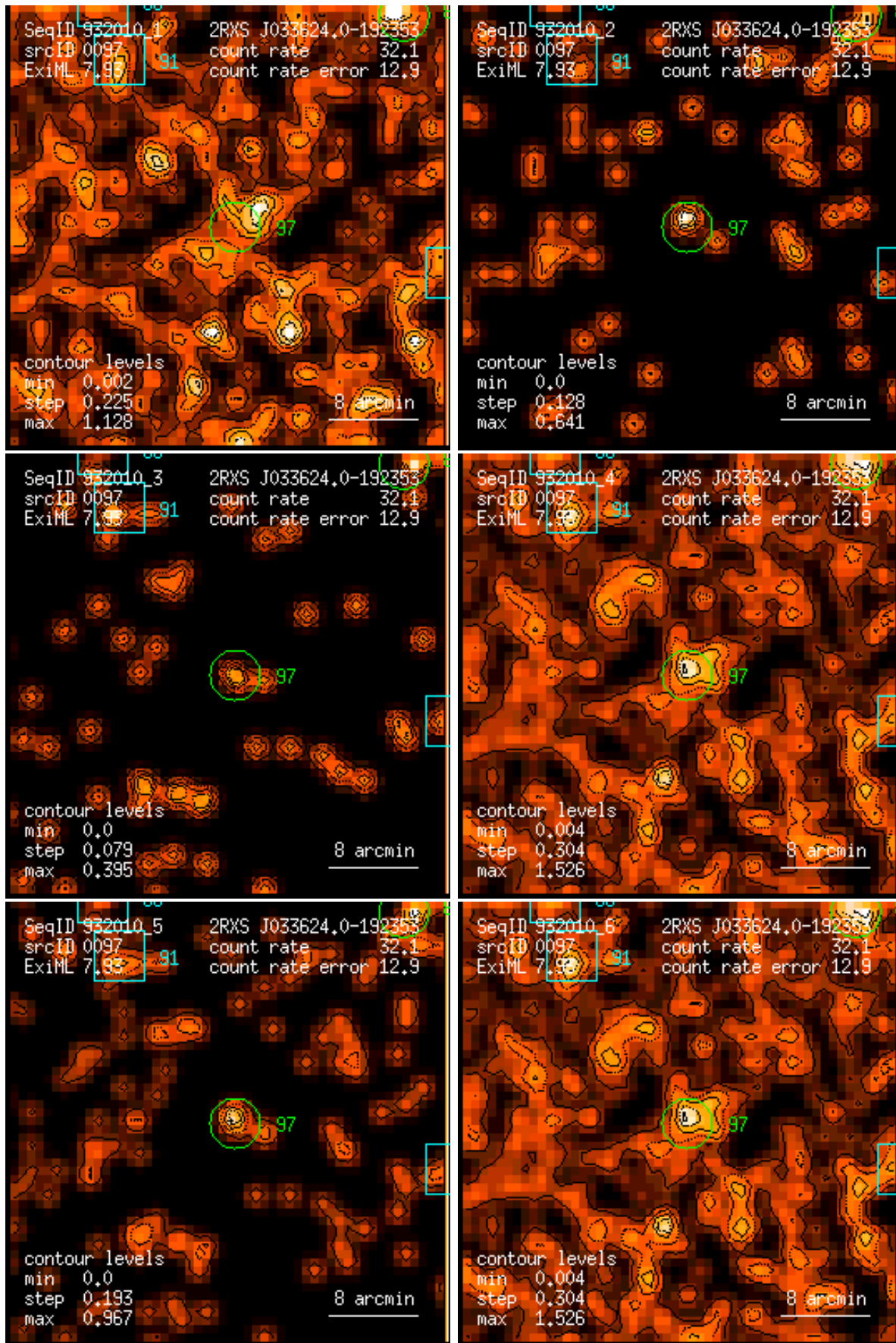
Figure 97: RASS 932010: detection 0097: band rate images, Gaussian filter: (1) PSPC channels 11 – 41, (2) 52 – 90, (3) 91 – 201, (4) 11 – 235, (5) 52 – 201, (6) 11 – 201. Broad band rates in counts/ks. Band rate contour levels in counts/ks/arcmin 2 .
