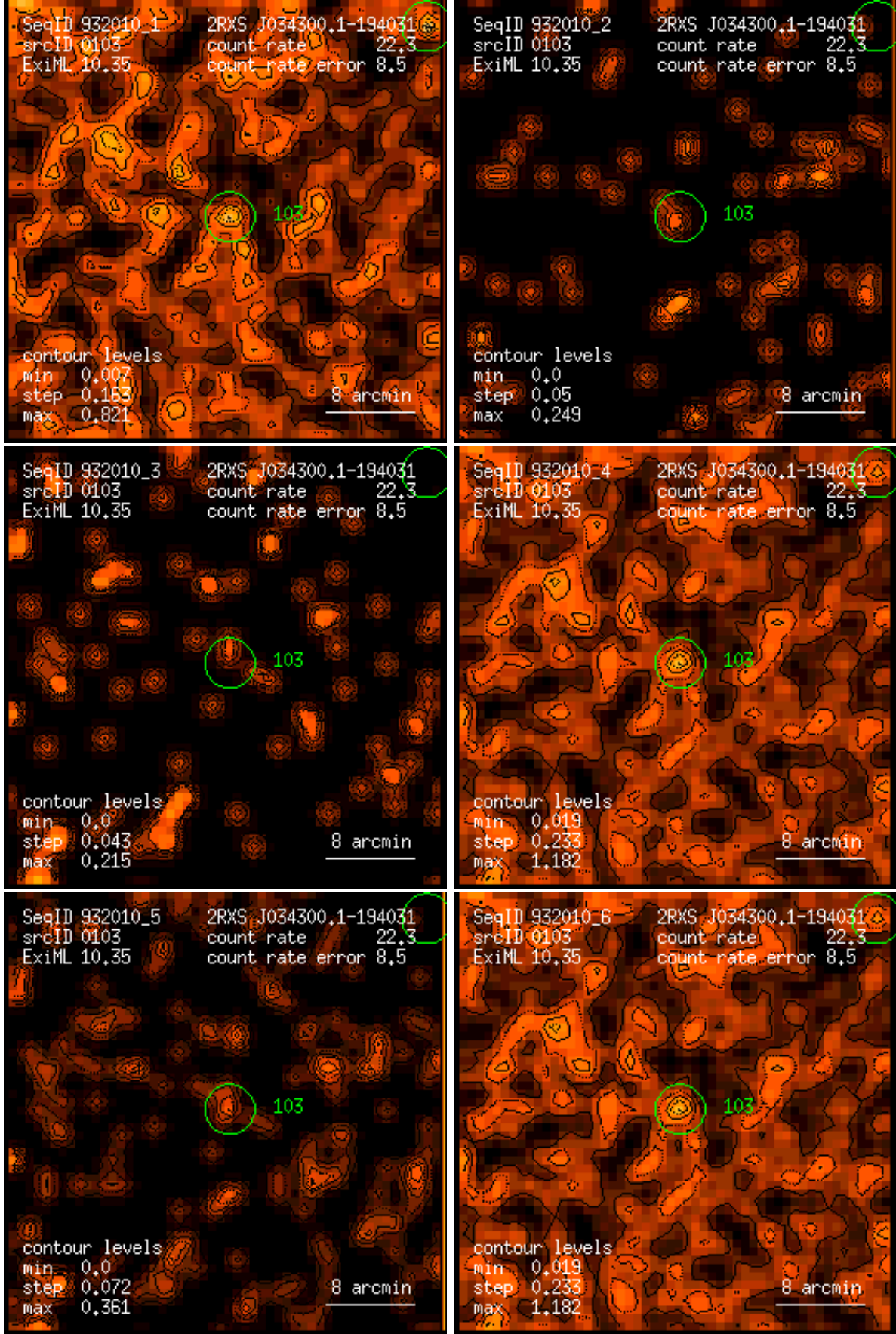
Figure 103: RASS 932010: detection 0103: band rate images, Gaussian filter: (1) PSPC channels 11 – 41, (2) 52 – 90, (3) 91 – 201, (4) 11 – 235, (5) 52 – 201, (6) 11 – 201. Broad band rates in counts/ks. Band rate contour levels in counts/ks/arcmin 2 .
