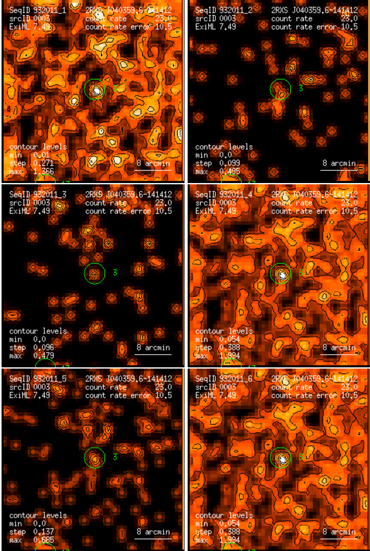
Figure 3: RASS 932011: detection 0003: band rate images, Gaussian filter: (1) PSPC channels 11 – 41, (2) 52 – 90, (3) 91 – 201, (4) 11 – 235, (5) 52 – 201, (6) 11 – 201. Broad band rates in counts/ks. Band rate contour levels in counts/ks/arcmin 2 .
