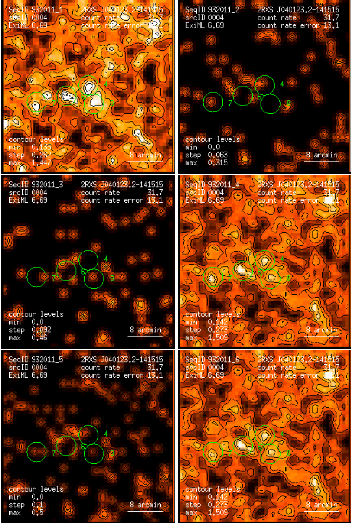
Figure 4: RASS 932011: detection 0004: band rate images, Gaussian filter: (1) PSPC channels 11 – 41, (2) 52 – 90, (3) 91 – 201, (4) 11 – 235, (5) 52 – 201, (6) 11 – 201. Broad band rates in counts/ks. Band rate contour levels in counts/ks/arcmin 2 .
