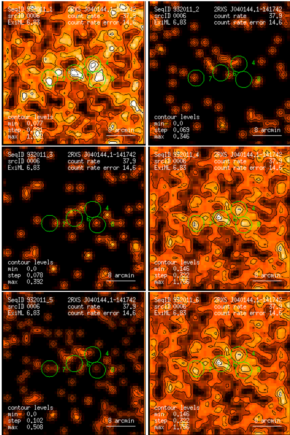
Figure 6: RASS 932011: detection 0006: band rate images, Gaussian filter: (1) PSPC channels 11 – 41, (2) 52 – 90, (3) 91 – 201, (4) 11 – 235, (5) 52 – 201, (6) 11 – 201. Broad band rates in counts/ks. Band rate contour levels in counts/ks/arcmin 2 .
