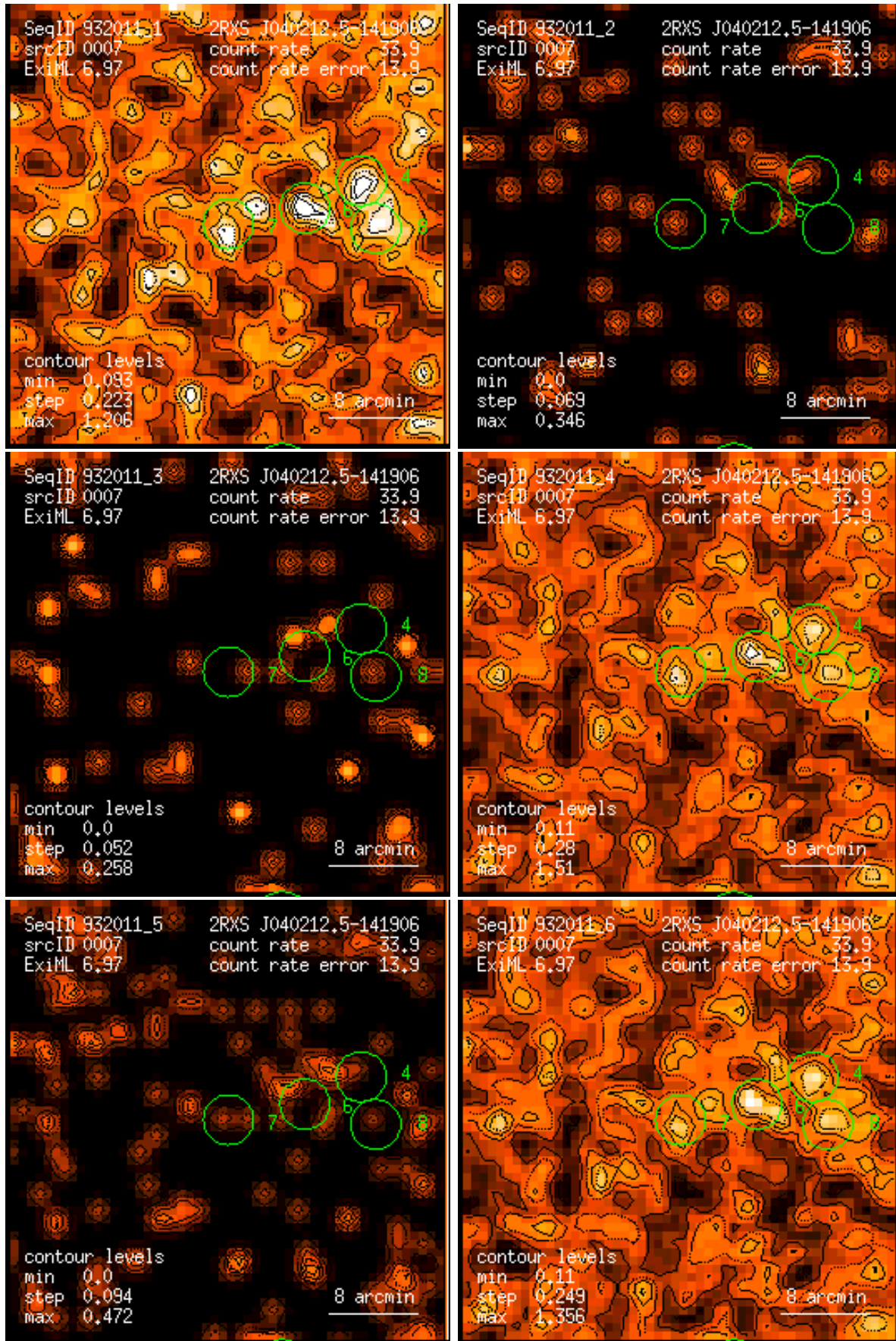
Figure 7: RASS 932011: detection 0007: band rate images, Gaussian filter: (1) PSPC channels 11 – 41, (2) 52 – 90, (3) 91 – 201, (4) 11 – 235, (5) 52 – 201, (6) 11 – 201. Broad band rates in counts/ks. Band rate contour levels in counts/ks/arcmin 2 .
