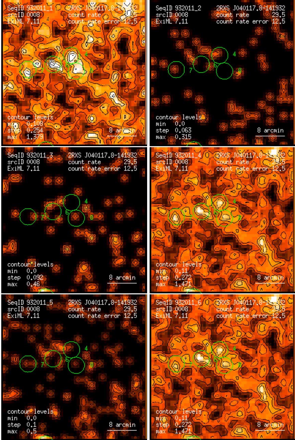
Figure 8: RASS 932011: detection 0008: band rate images, Gaussian filter: (1) PSPC channels 11 – 41, (2) 52 – 90, (3) 91 – 201, (4) 11 – 235, (5) 52 – 201, (6) 11 – 201. Broad band rates in counts/ks. Band rate contour levels in counts/ks/arcmin 2 .
