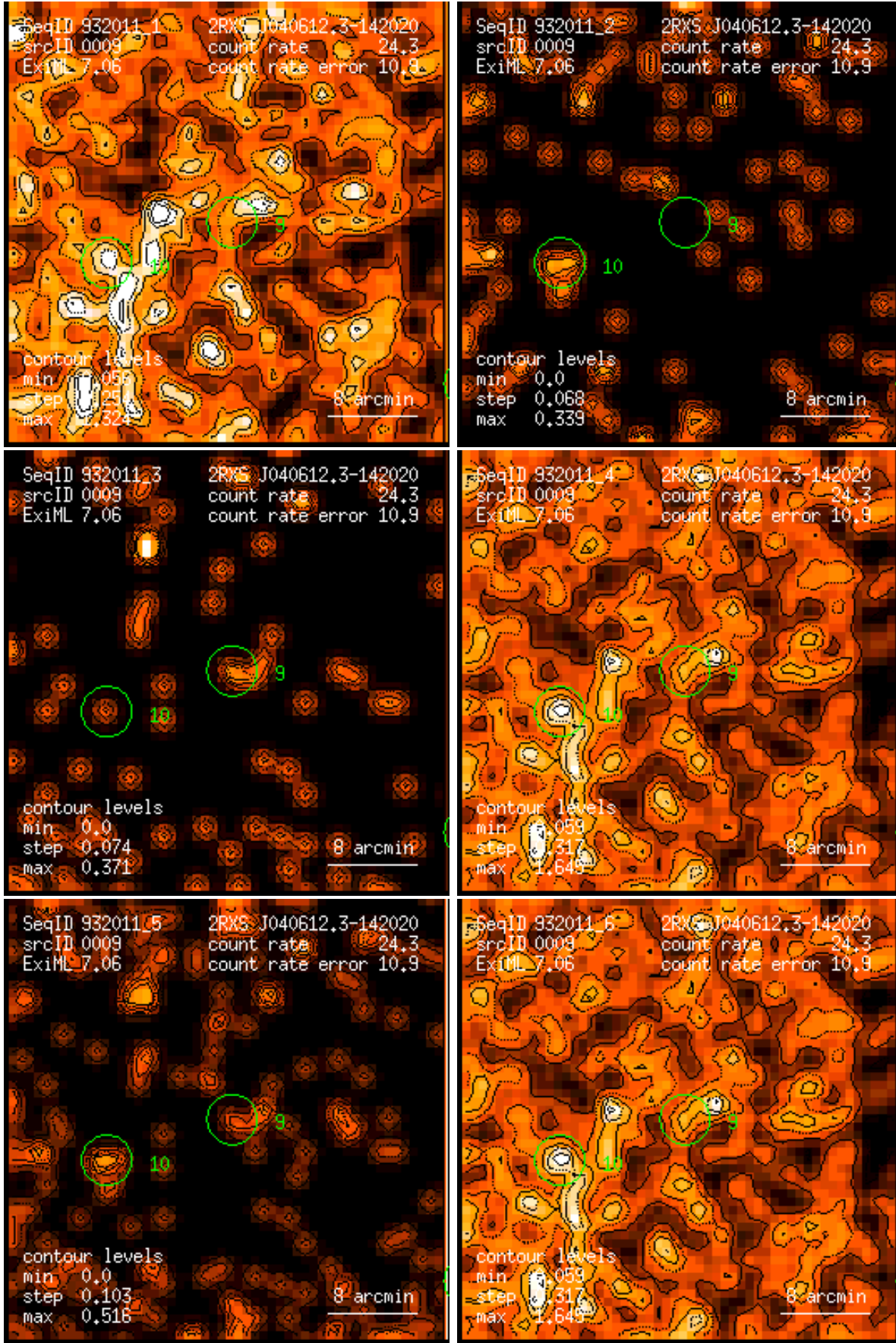
Figure 9: RASS 932011: detection 0009: band rate images, Gaussian filter: (1) PSPC channels 11 – 41, (2) 52 – 90, (3) 91 – 201, (4) 11 – 235, (5) 52 – 201, (6) 11 – 201. Broad band rates in counts/ks. Band rate contour levels in counts/ks/arcmin 2 .
