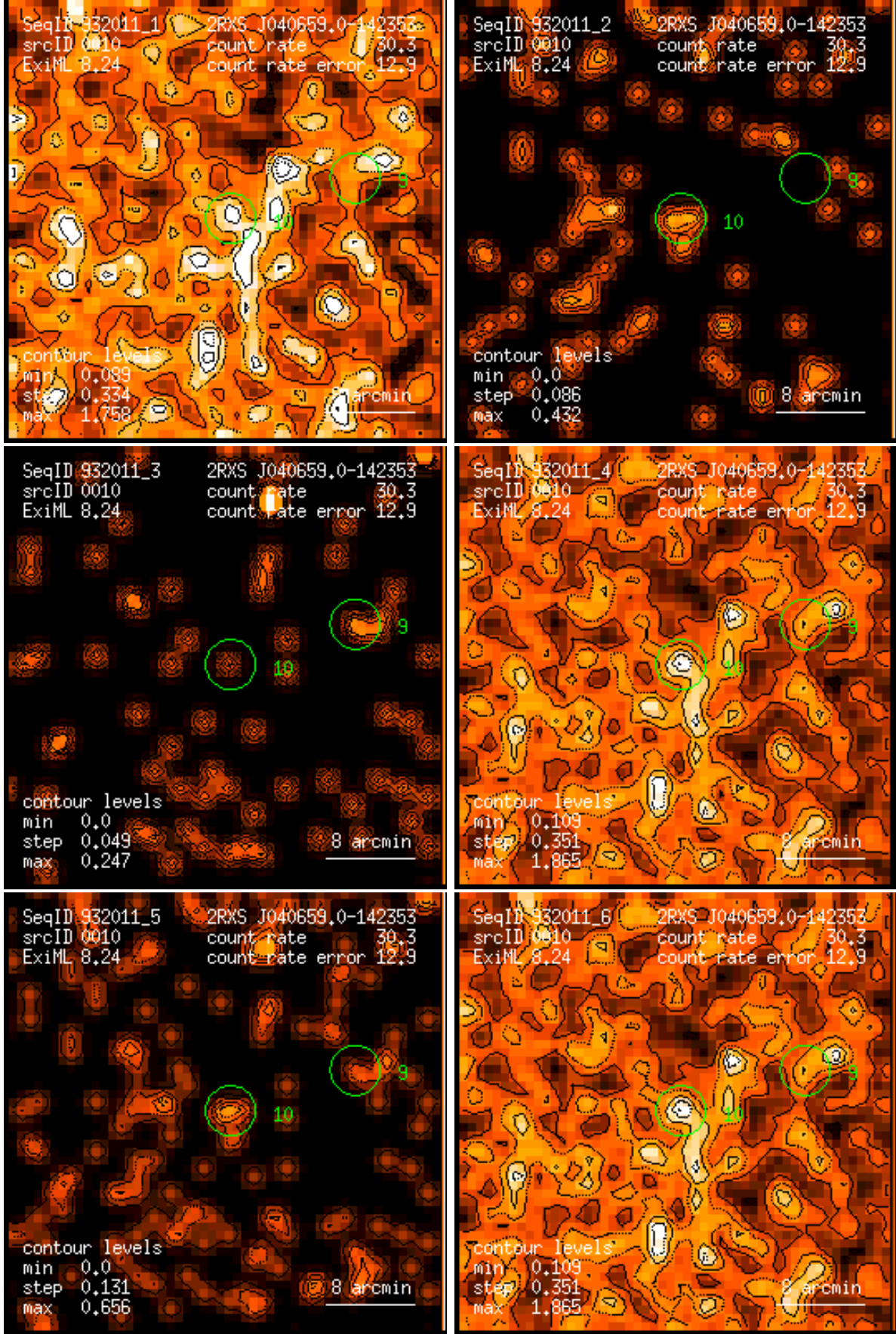
Figure 10: RASS 932011: detection 0010: band rate images, Gaussian filter: (1) PSPC channels 11 – 41, (2) 52 – 90, (3) 91 – 201, (4) 11 – 235, (5) 52 – 201, (6) 11 – 201. Broad band rates in counts/ks. Band rate contour levels in counts/ks/arcmin 2 .
