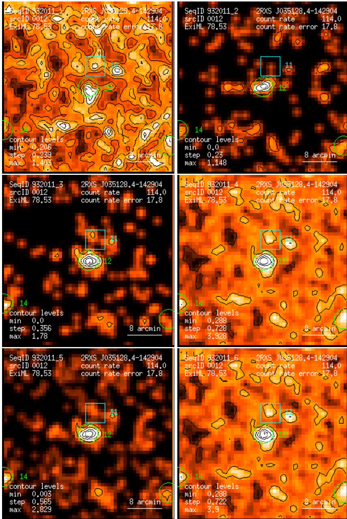
Figure 12: RASS 932011: detection 0012: band rate images, Gaussian filter: (1) PSPC channels 11 – 41, (2) 52 – 90, (3) 91 – 201, (4) 11 – 235, (5) 52 – 201, (6) 11 – 201. Broad band rates in counts/ks. Band rate contour levels in counts/ks/arcmin 2 .
