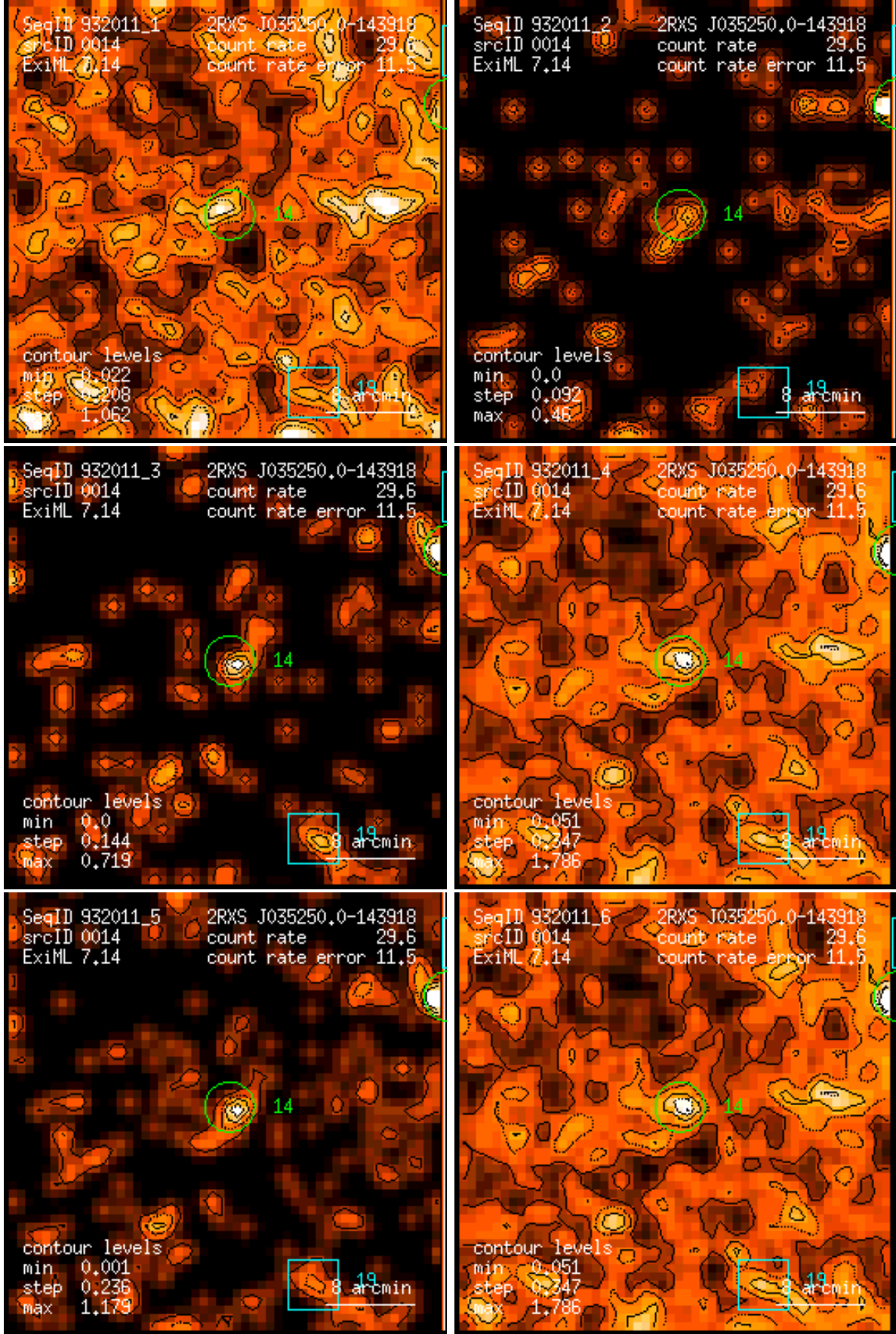
Figure 14: RASS 932011: detection 0014: band rate images, Gaussian filter: (1) PSPC channels 11 – 41, (2) 52 – 90, (3) 91 – 201, (4) 11 – 235, (5) 52 – 201, (6) 11 – 201. Broad band rates in counts/ks. Band rate contour levels in counts/ks/arcmin 2 .
