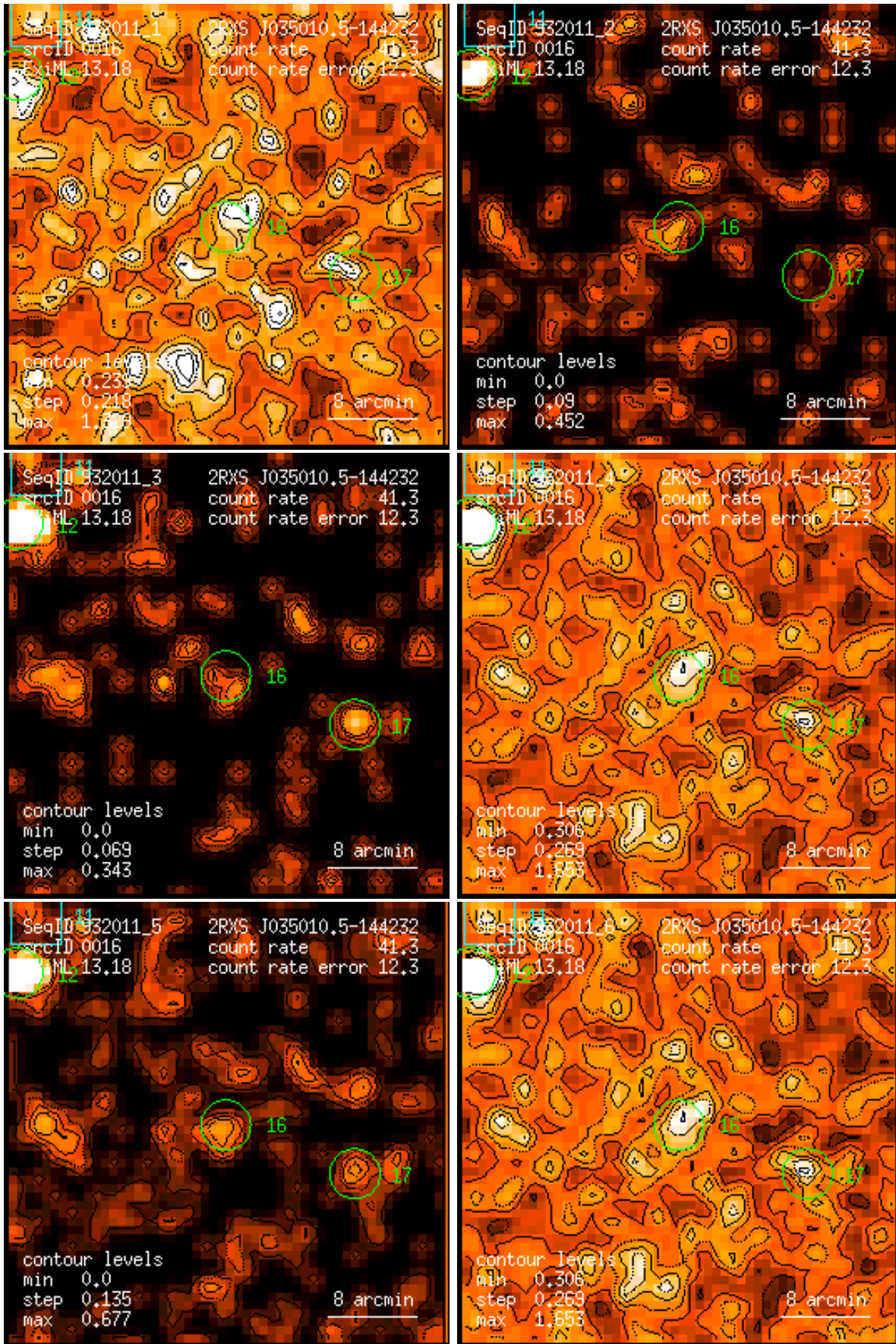
Figure 16: RASS 932011: detection 0016: band rate images, Gaussian filter: (1) PSPC channels 11 – 41, (2) 52 – 90, (3) 91 – 201, (4) 11 – 235, (5) 52 – 201, (6) 11 – 201. Broad band rates in counts/ks. Band rate contour levels in counts/ks/arcmin 2 .
