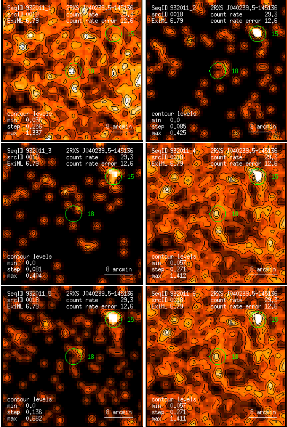
Figure 18: RASS 932011: detection 0018: band rate images, Gaussian filter: (1) PSPC channels 11 – 41, (2) 52 – 90, (3) 91 – 201, (4) 11 – 235, (5) 52 – 201, (6) 11 – 201. Broad band rates in counts/ks. Band rate contour levels in counts/ks/arcmin 2 .
