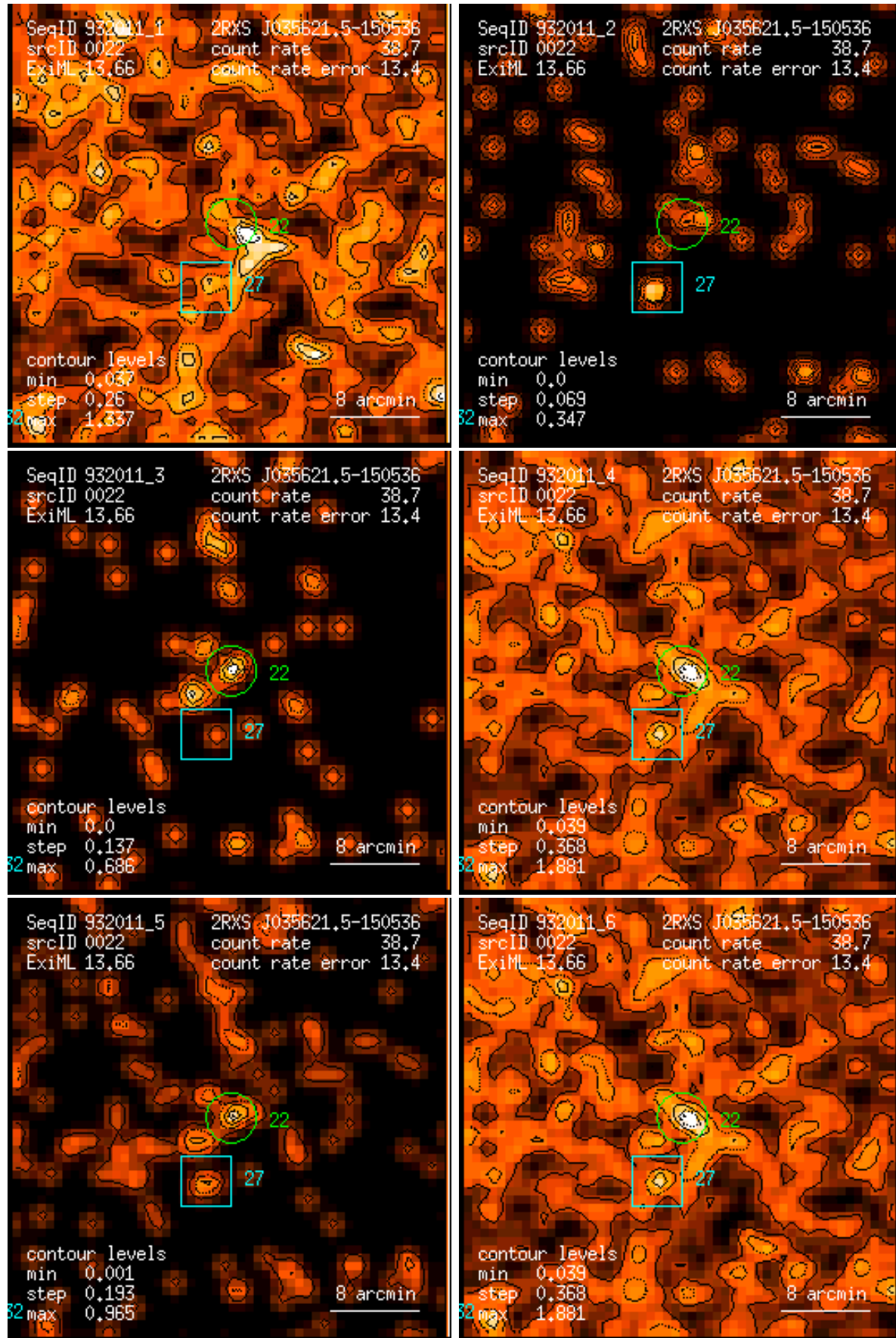
Figure 22: RASS 932011: detection 0022: band rate images, Gaussian filter: (1) PSPC channels 11 – 41, (2) 52 – 90, (3) 91 – 201, (4) 11 – 235, (5) 52 – 201, (6) 11 – 201. Broad band rates in counts/ks. Band rate contour levels in counts/ks/arcmin 2 .
