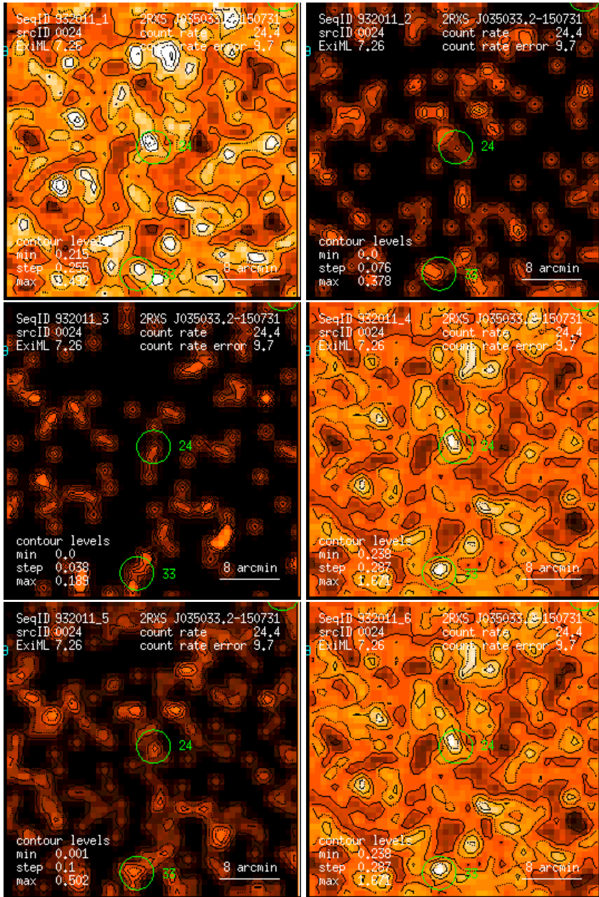
Figure 24: RASS 932011: detection 0024: band rate images, Gaussian filter: (1) PSPC channels 11 – 41, (2) 52 – 90, (3) 91 – 201, (4) 11 – 235, (5) 52 – 201, (6) 11 – 201. Broad band rates in counts/ks. Band rate contour levels in counts/ks/arcmin 2 .
