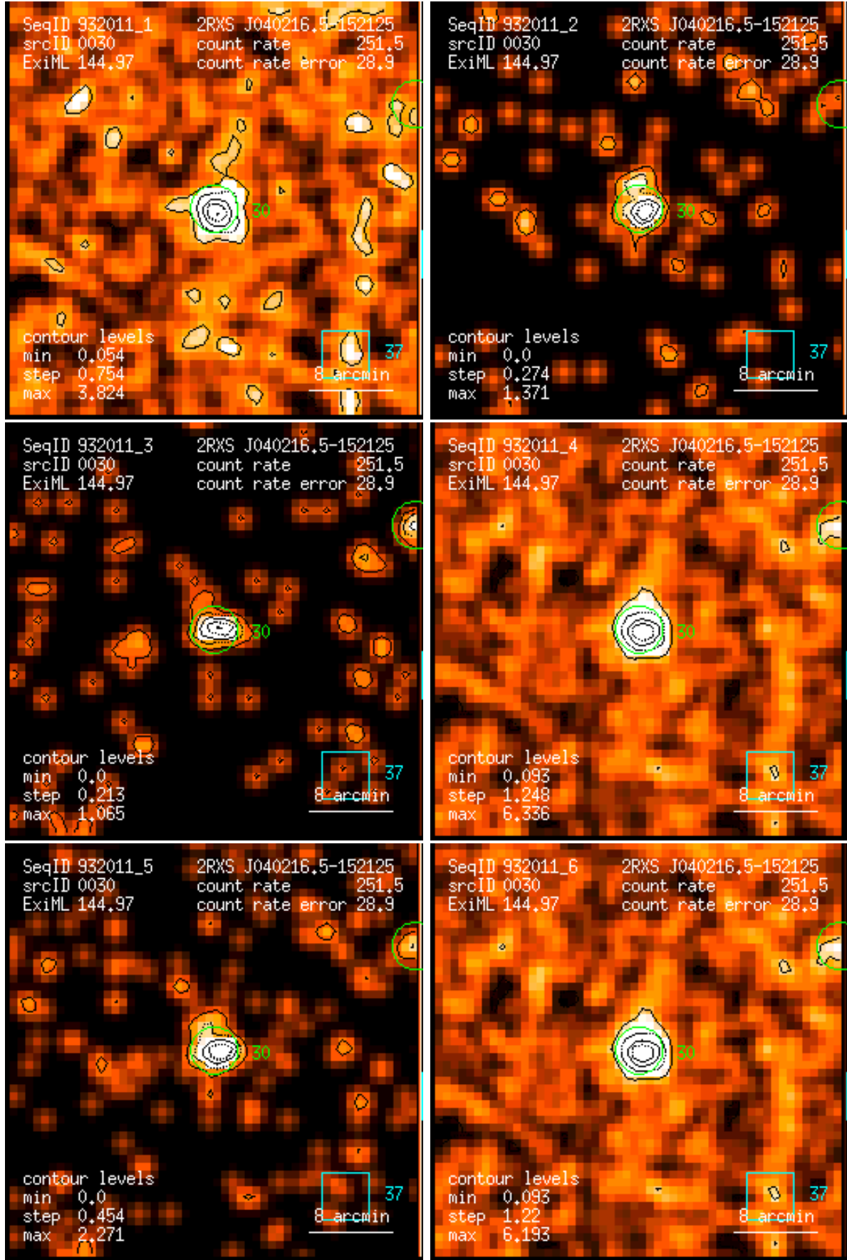
Figure 30: RASS 932011: detection 0030: band rate images, Gaussian filter: (1) PSPC channels 11 – 41, (2) 52 – 90, (3) 91 – 201, (4) 11 – 235, (5) 52 – 201, (6) 11 – 201. Broad band rates in counts/ks. Band rate contour levels in counts/ks/arcmin 2 .
