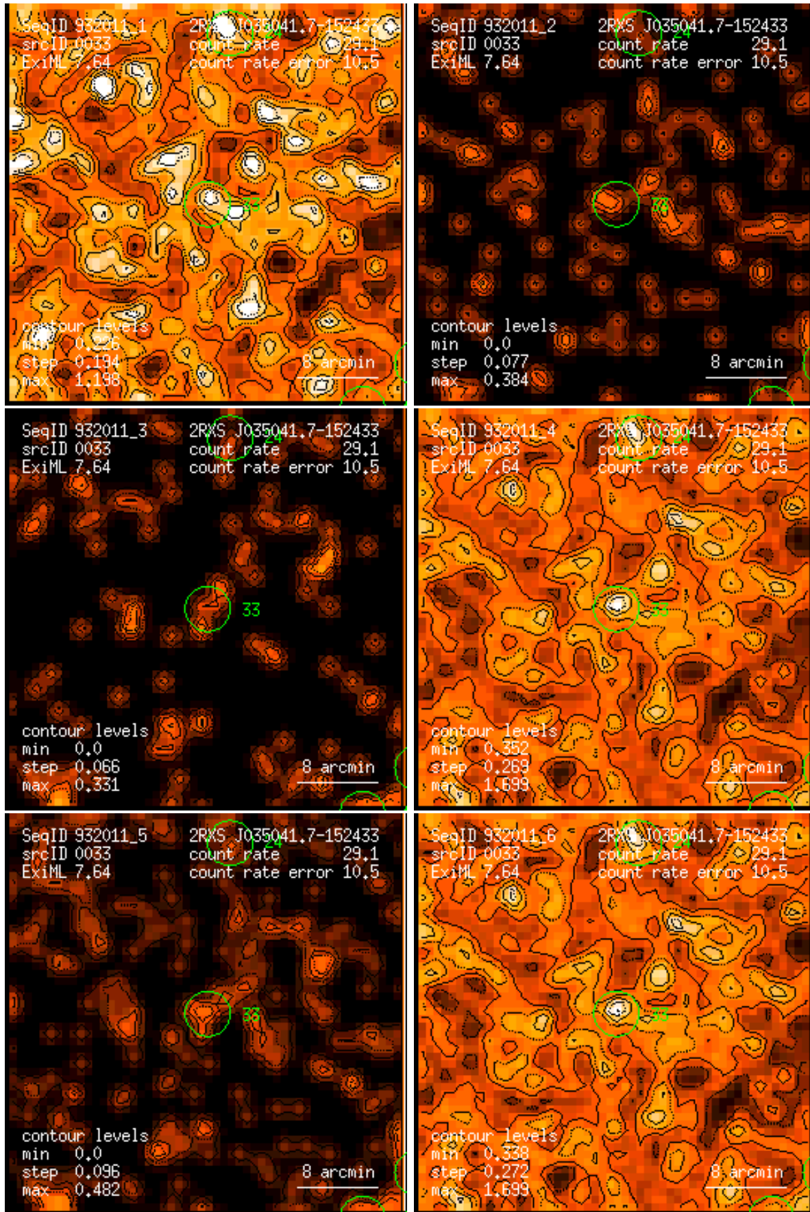
Figure 33: RASS 932011: detection 0033: band rate images, Gaussian filter: (1) PSPC channels 11 – 41, (2) 52 – 90, (3) 91 – 201, (4) 11 – 235, (5) 52 – 201, (6) 11 – 201. Broad band rates in counts/ks. Band rate contour levels in counts/ks/arcmin 2 .
