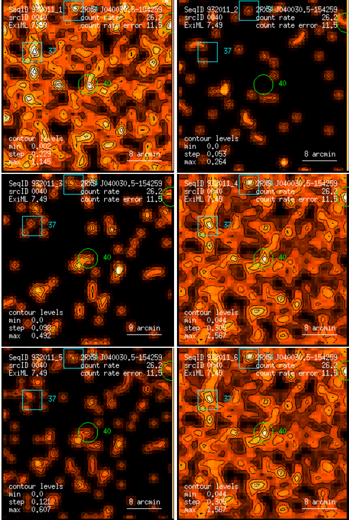
Figure 40: RASS 932011: detection 0040: band rate images, Gaussian filter: (1) PSPC channels 11 – 41, (2) 52 – 90, (3) 91 – 201, (4) 11 – 235, (5) 52 – 201, (6) 11 – 201. Broad band rates in counts/ks. Band rate contour levels in counts/ks/arcmin 2 .
