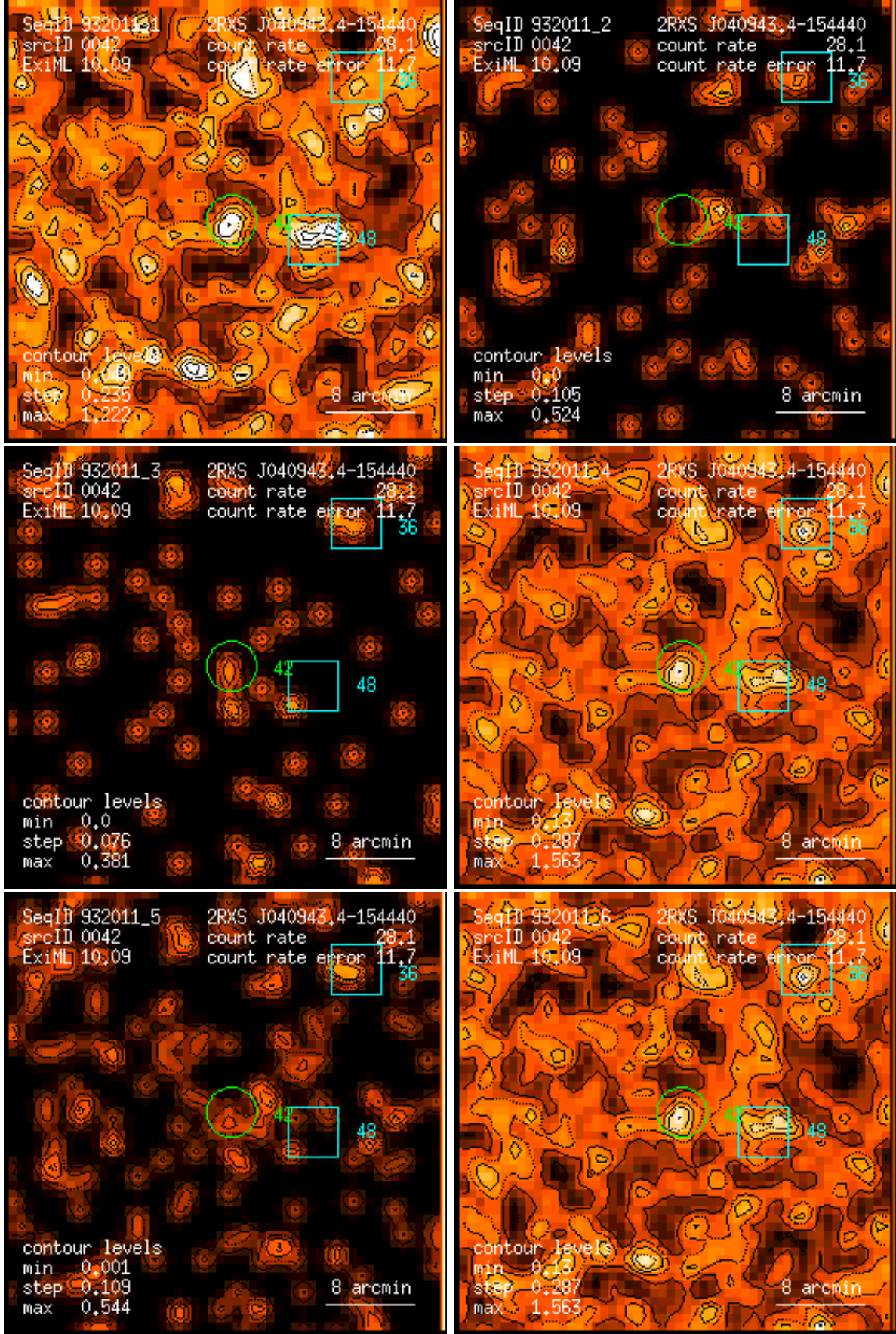
Figure 42: RASS 932011: detection 0042: band rate images, Gaussian filter: (1) PSPC channels 11 – 41, (2) 52 – 90, (3) 91 – 201, (4) 11 – 235, (5) 52 – 201, (6) 11 – 201. Broad band rates in counts/ks. Band rate contour levels in counts/ks/arcmin 2 .
