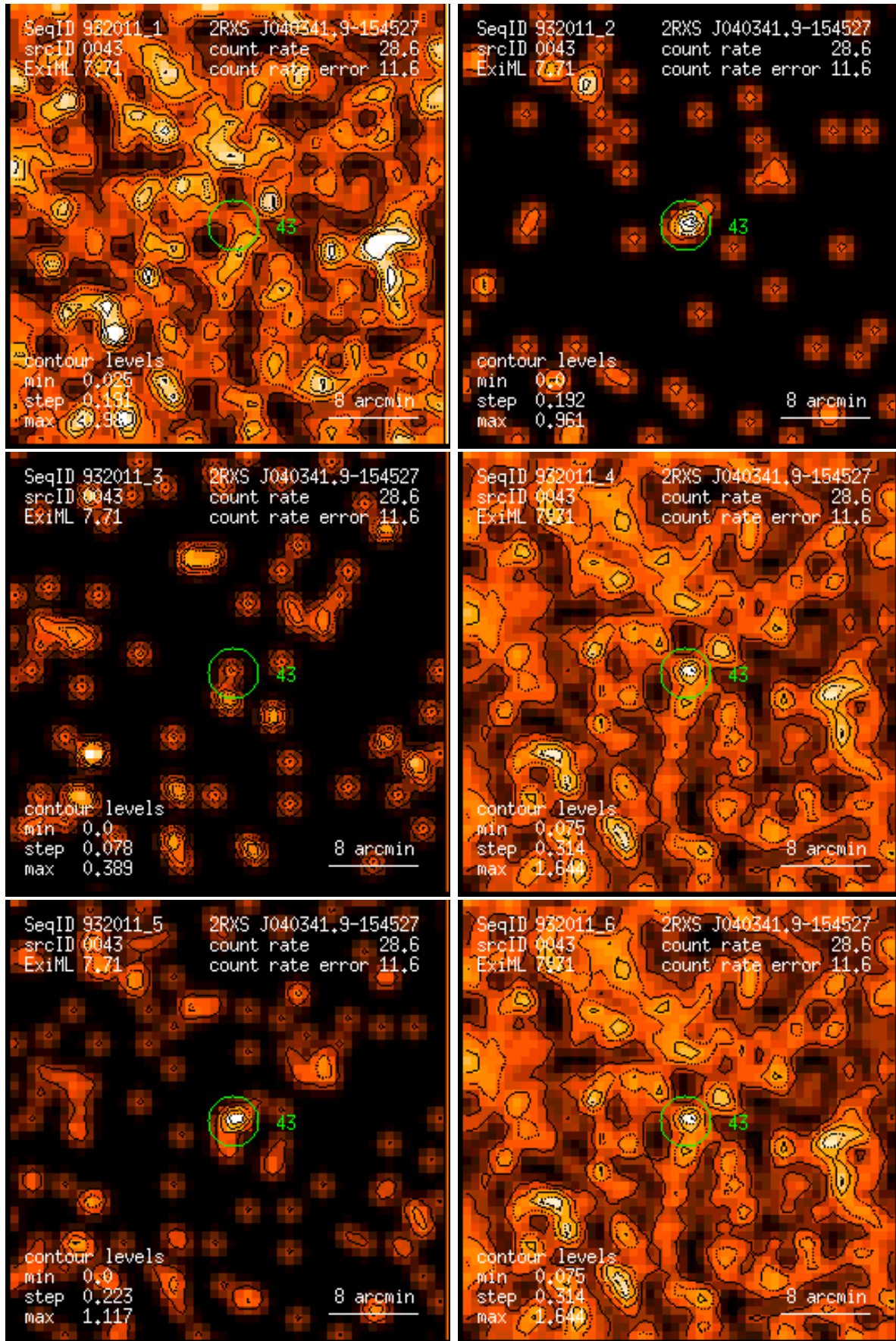
Figure 43: RASS 932011: detection 0043: band rate images, Gaussian filter: (1) PSPC channels 11 – 41, (2) 52 – 90, (3) 91 – 201, (4) 11 – 235, (5) 52 – 201, (6) 11 – 201. Broad band rates in counts/ks. Band rate contour levels in counts/ks/arcmin 2 .
