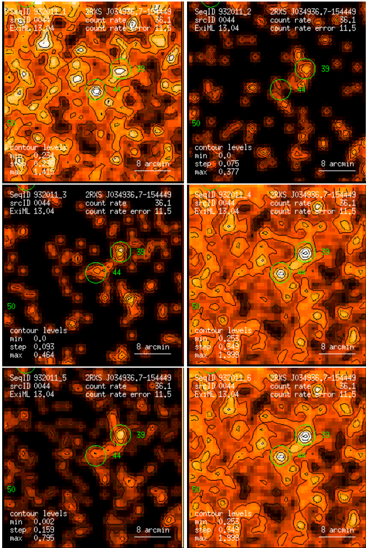
Figure 44: RASS 932011: detection 0044: band rate images, Gaussian filter: (1) PSPC channels 11 – 41, (2) 52 – 90, (3) 91 – 201, (4) 11 – 235, (5) 52 – 201, (6) 11 – 201. Broad band rates in counts/ks. Band rate contour levels in counts/ks/arcmin 2 .
