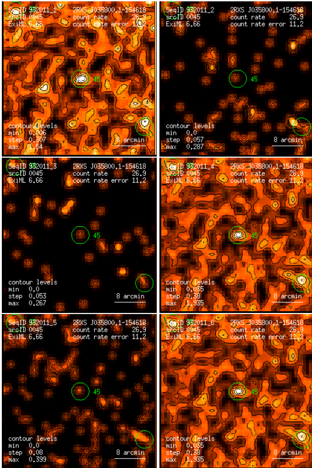
Figure 45: RASS 932011: detection 0045: band rate images, Gaussian filter: (1) PSPC channels 11 – 41, (2) 52 – 90, (3) 91 – 201, (4) 11 – 235, (5) 52 – 201, (6) 11 – 201. Broad band rates in counts/ks. Band rate contour levels in counts/ks/arcmin 2 .
