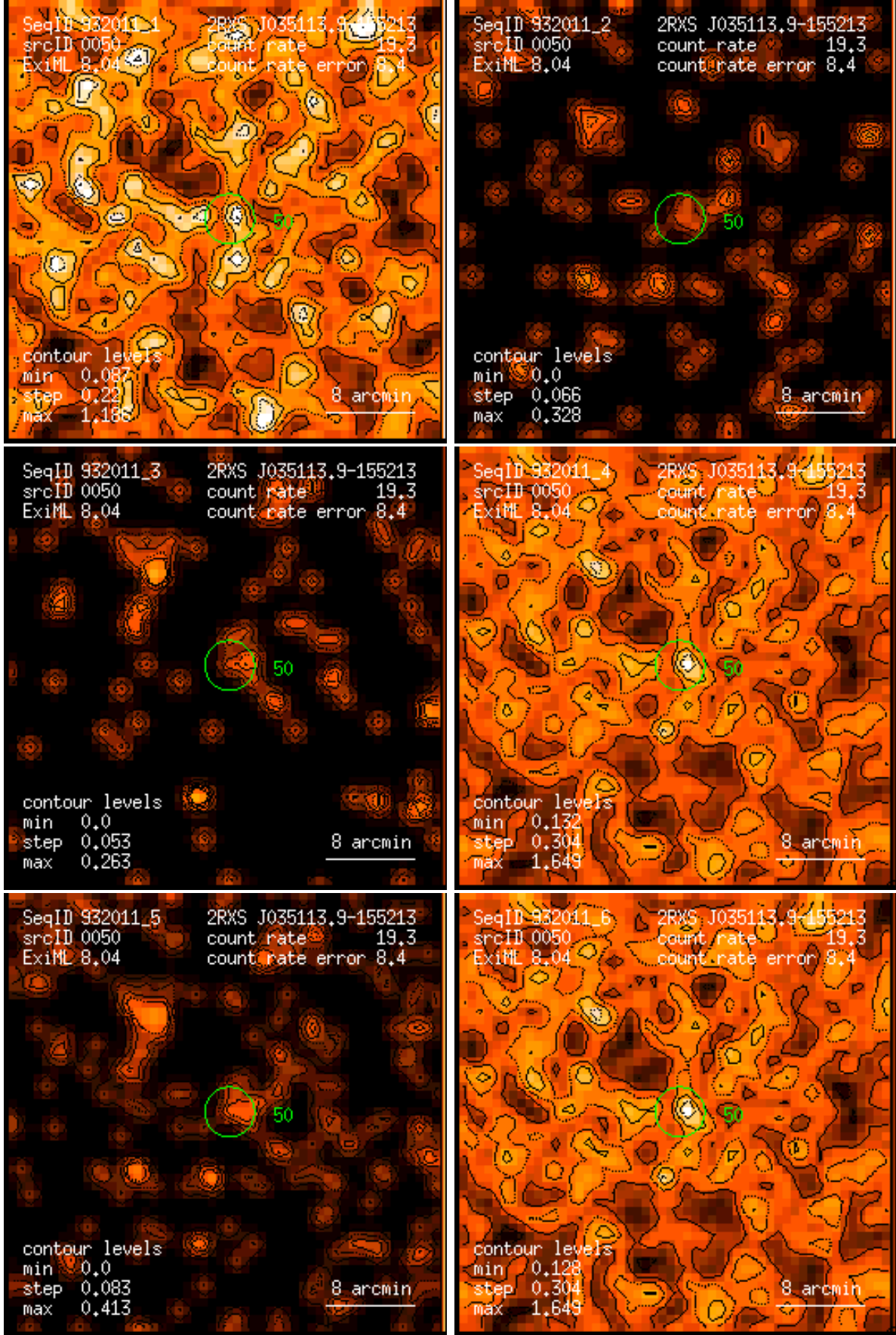
Figure 50: RASS 932011: detection 0050: band rate images, Gaussian filter: (1) PSPC channels 11 – 41, (2) 52 – 90, (3) 91 – 201, (4) 11 – 235, (5) 52 – 201, (6) 11 – 201. Broad band rates in counts/ks. Band rate contour levels in counts/ks/arcmin 2 .
