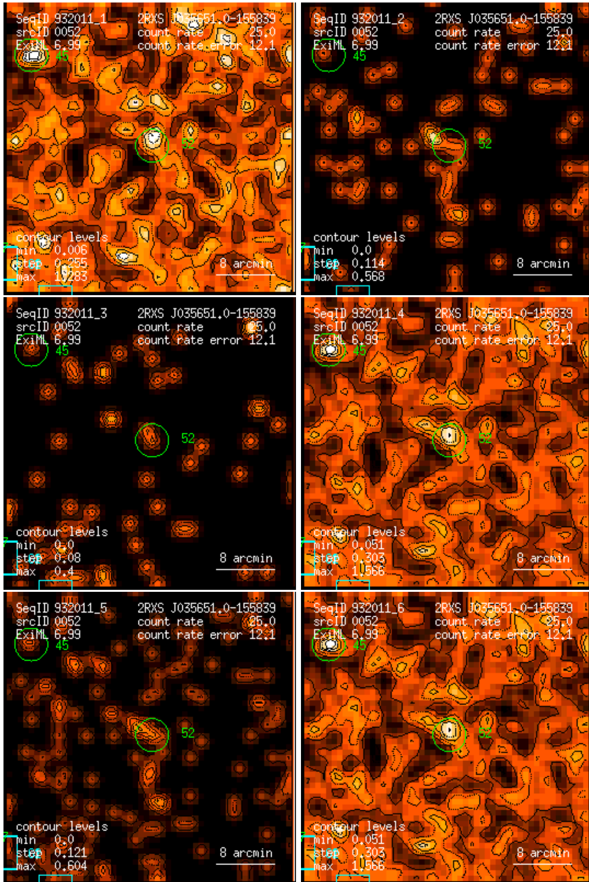
Figure 52: RASS 932011: detection 0052: band rate images, Gaussian filter: (1) PSPC channels 11 – 41, (2) 52 – 90, (3) 91 – 201, (4) 11 – 235, (5) 52 – 201, (6) 11 – 201. Broad band rates in counts/ks. Band rate contour levels in counts/ks/arcmin 2 .
