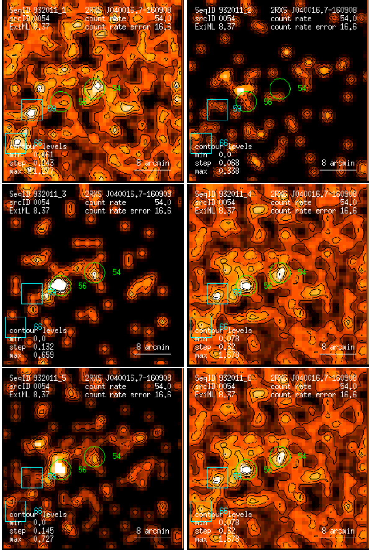
Figure 54: RASS 932011: detection 0054: band rate images, Gaussian filter: (1) PSPC channels 11 – 41, (2) 52 – 90, (3) 91 – 201, (4) 11 – 235, (5) 52 – 201, (6) 11 – 201. Broad band rates in counts/ks. Band rate contour levels in counts/ks/arcmin 2 .
