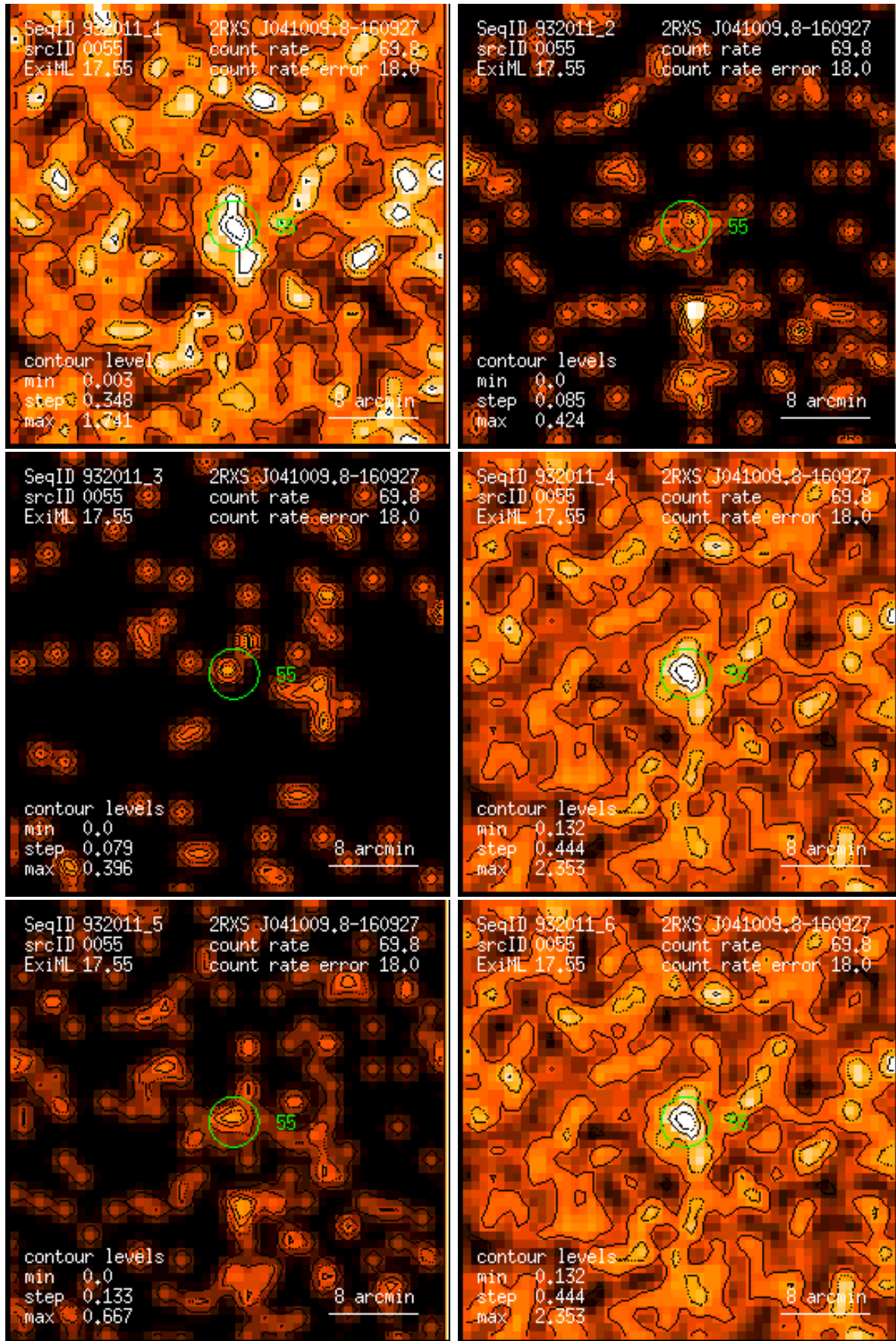
Figure 55: RASS 932011: detection 0055: band rate images, Gaussian filter: (1) PSPC channels 11 – 41, (2) 52 – 90, (3) 91 – 201, (4) 11 – 235, (5) 52 – 201, (6) 11 – 201. Broad band rates in counts/ks. Band rate contour levels in counts/ks/arcmin 2 .
