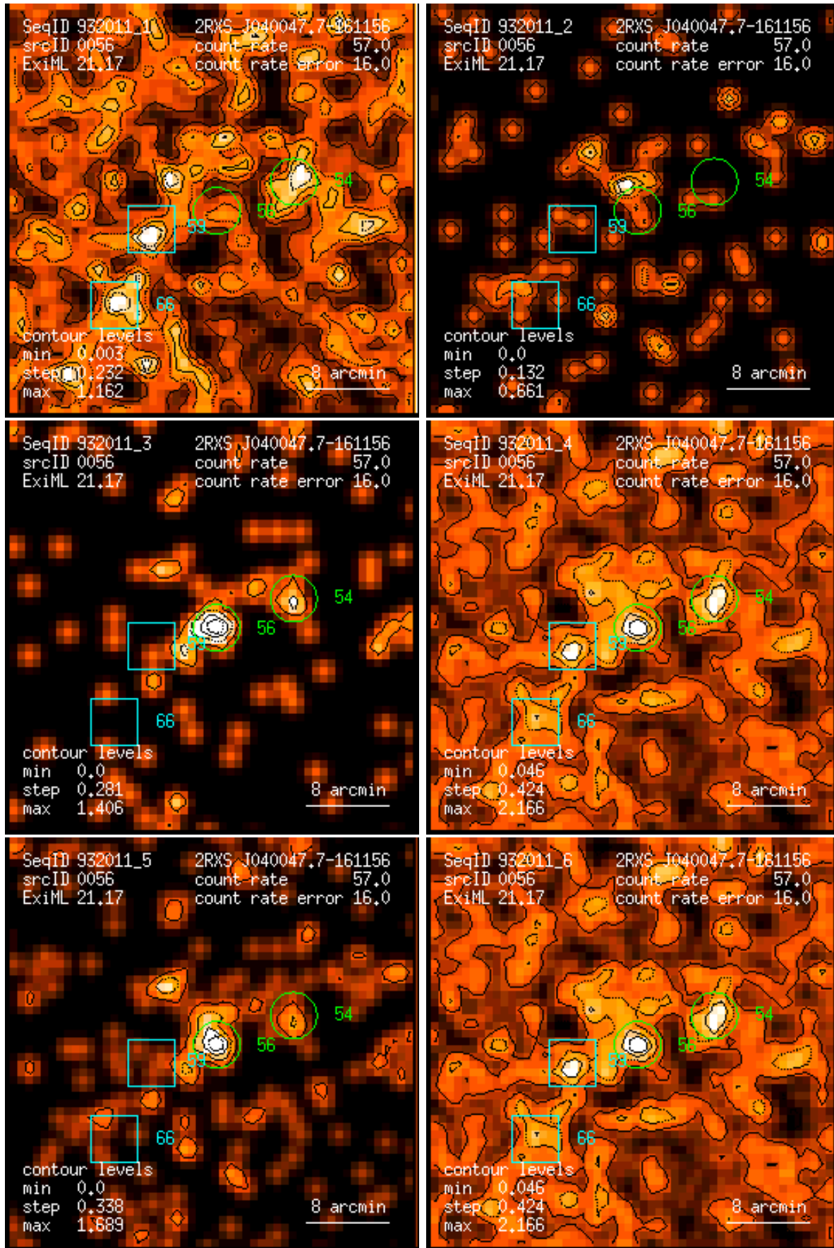
Figure 56: RASS 932011: detection 0056: band rate images, Gaussian filter: (1) PSPC channels 11 – 41, (2) 52 – 90, (3) 91 – 201, (4) 11 – 235, (5) 52 – 201, (6) 11 – 201. Broad band rates in counts/ks. Band rate contour levels in counts/ks/arcmin 2 .
