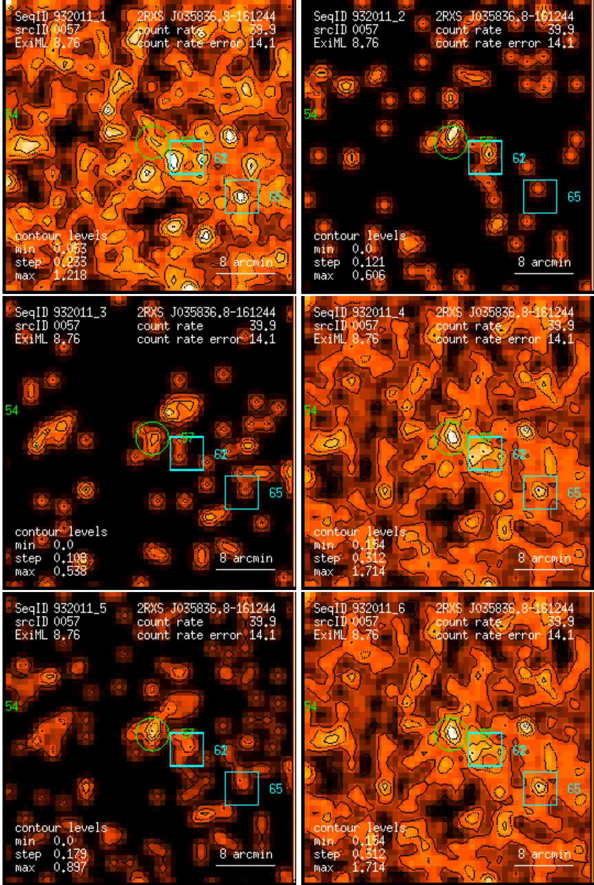
Figure 57: RASS 932011: detection 0057: band rate images, Gaussian filter: (1) PSPC channels 11 – 41, (2) 52 – 90, (3) 91 – 201, (4) 11 – 235, (5) 52 – 201, (6) 11 – 201. Broad band rates in counts/ks. Band rate contour levels in counts/ks/arcmin 2 .
