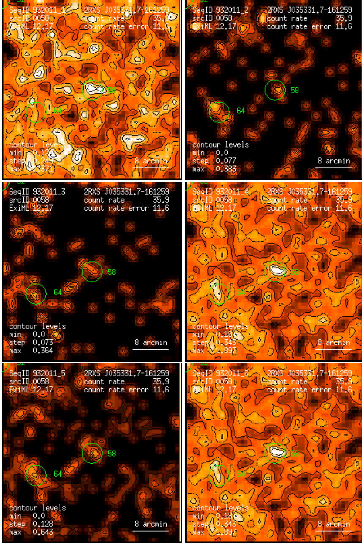
Figure 58: RASS 932011: detection 0058: band rate images, Gaussian filter: (1) PSPC channels 11 – 41, (2) 52 – 90, (3) 91 – 201, (4) 11 – 235, (5) 52 – 201, (6) 11 – 201. Broad band rates in counts/ks. Band rate contour levels in counts/ks/arcmin 2 .
