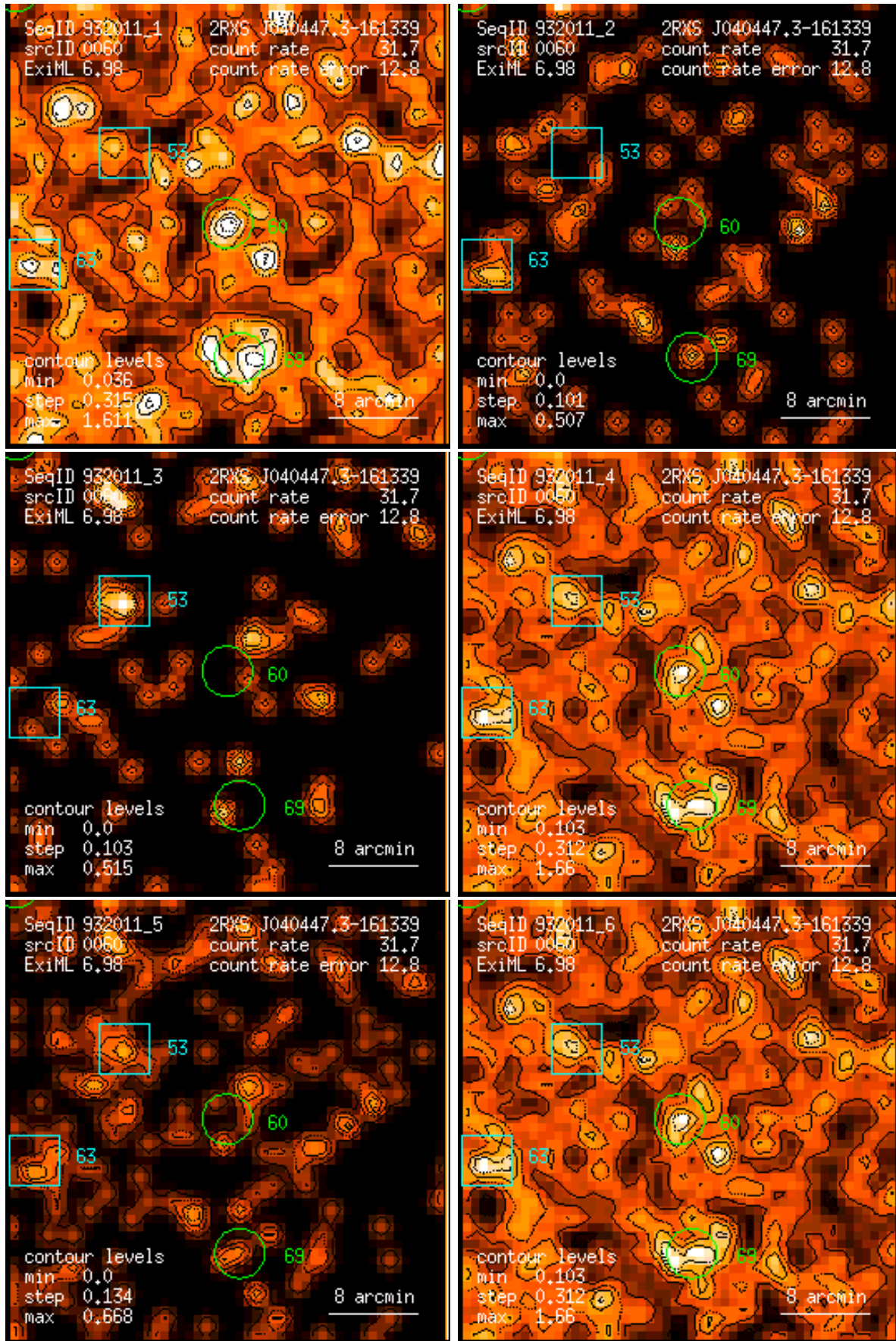
Figure 60: RASS 932011: detection 0060: band rate images, Gaussian filter: (1) PSPC channels 11 – 41, (2) 52 – 90, (3) 91 – 201, (4) 11 – 235, (5) 52 – 201, (6) 11 – 201. Broad band rates in counts/ks. Band rate contour levels in counts/ks/arcmin 2 .
