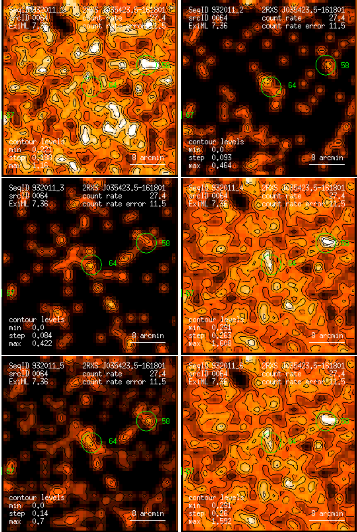
Figure 64: RASS 932011: detection 0064: band rate images, Gaussian filter: (1) PSPC channels 11 – 41, (2) 52 – 90, (3) 91 – 201, (4) 11 – 235, (5) 52 – 201, (6) 11 – 201. Broad band rates in counts/ks. Band rate contour levels in counts/ks/arcmin 2 .
