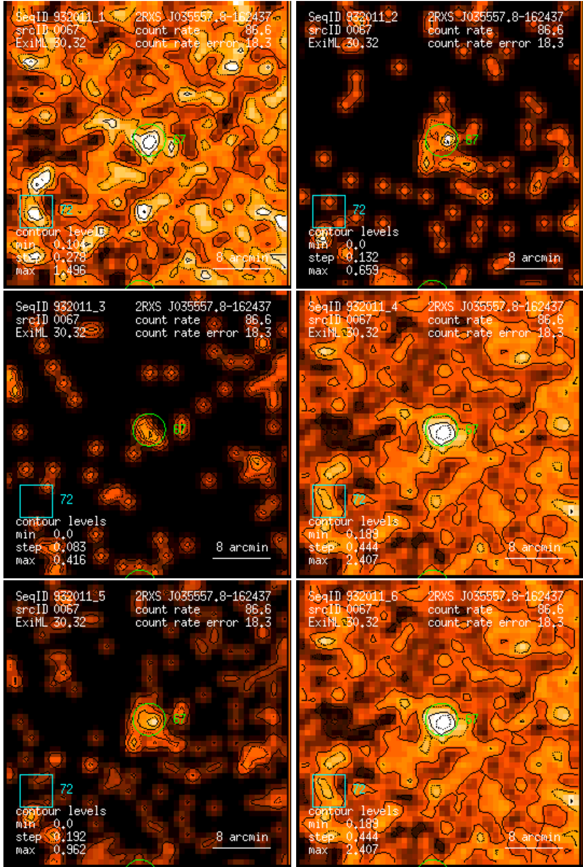
Figure 67: RASS 932011: detection 0067: band rate images, Gaussian filter: (1) PSPC channels 11 – 41, (2) 52 – 90, (3) 91 – 201, (4) 11 – 235, (5) 52 – 201, (6) 11 – 201. Broad band rates in counts/ks. Band rate contour levels in counts/ks/arcmin 2 .
