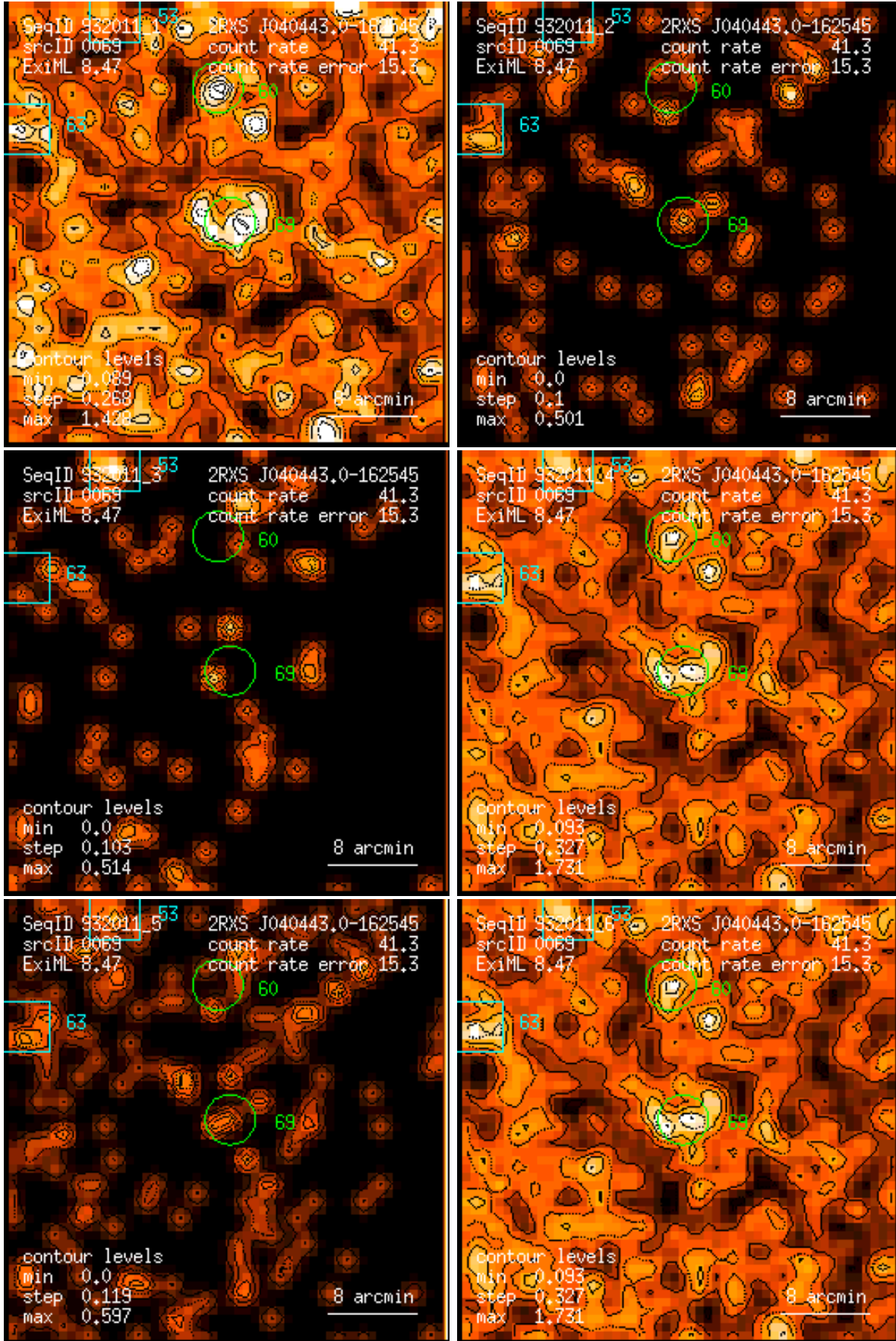
Figure 69: RASS 932011: detection 0069: band rate images, Gaussian filter: (1) PSPC channels 11 – 41, (2) 52 – 90, (3) 91 – 201, (4) 11 – 235, (5) 52 – 201, (6) 11 – 201. Broad band rates in counts/ks. Band rate contour levels in counts/ks/arcmin 2 .
