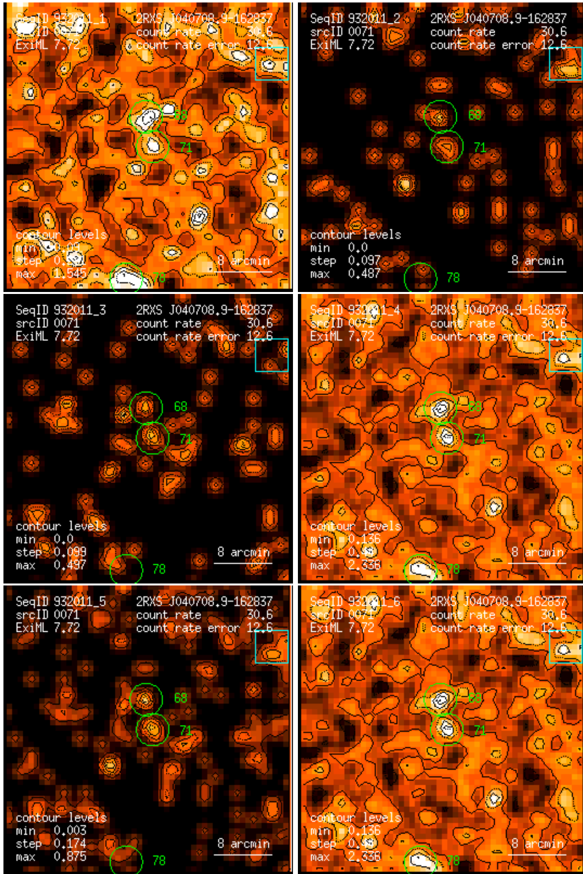
Figure 71: RASS 932011: detection 0071: band rate images, Gaussian filter: (1) PSPC channels 11 – 41, (2) 52 – 90, (3) 91 – 201, (4) 11 – 235, (5) 52 – 201, (6) 11 – 201. Broad band rates in counts/ks. Band rate contour levels in counts/ks/arcmin 2 .
