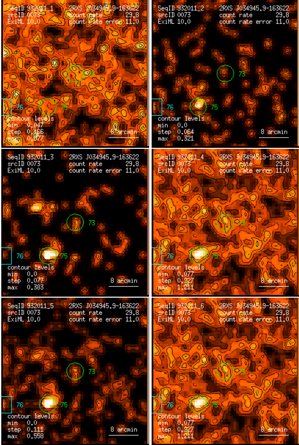
Figure 73: RASS 932011: detection 0073: band rate images, Gaussian filter: (1) PSPC channels 11 – 41, (2) 52 – 90, (3) 91 – 201, (4) 11 – 235, (5) 52 – 201, (6) 11 – 201. Broad band rates in counts/ks. Band rate contour levels in counts/ks/arcmin 2 .
