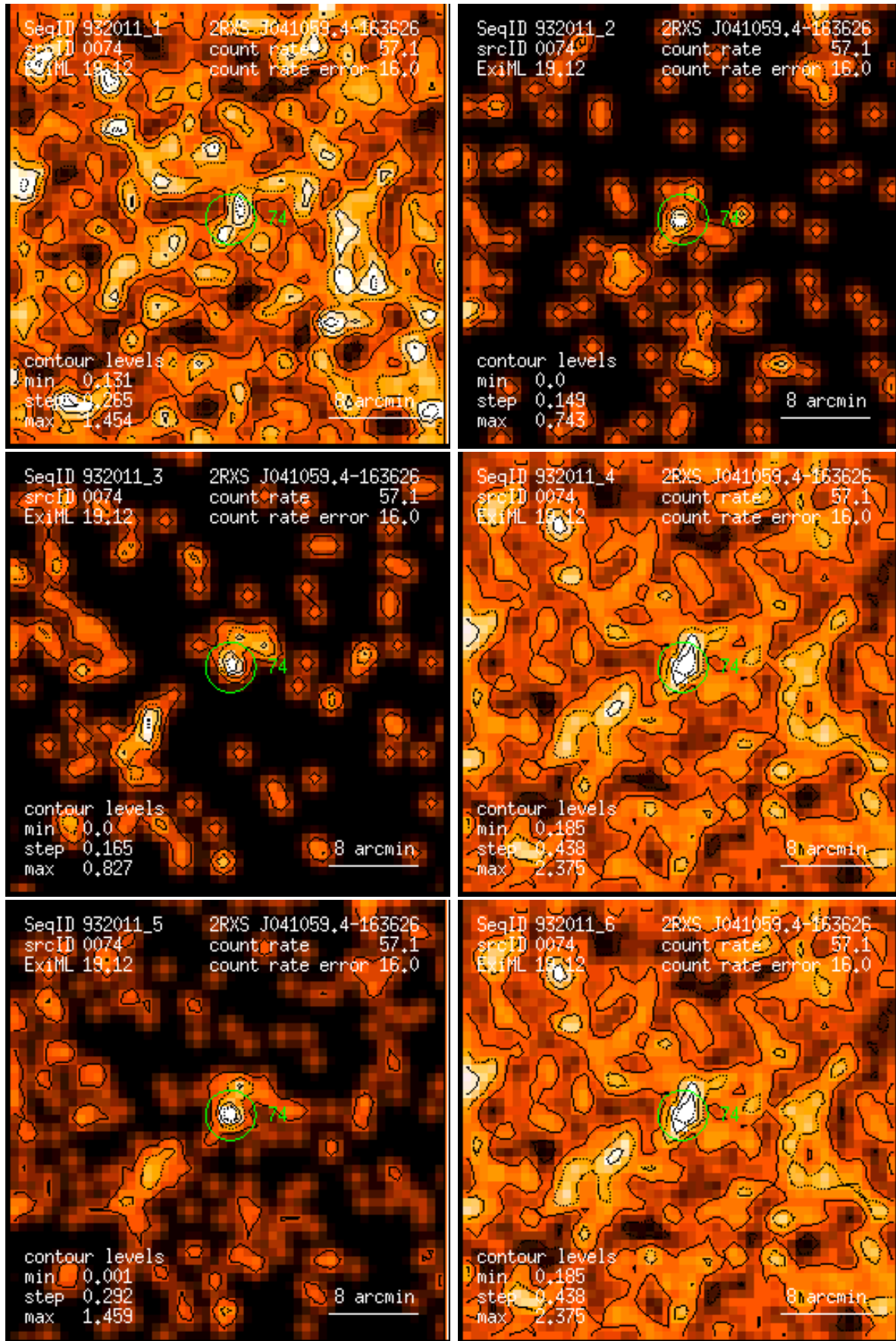
Figure 74: RASS 932011: detection 0074: band rate images, Gaussian filter: (1) PSPC channels 11 – 41, (2) 52 – 90, (3) 91 – 201, (4) 11 – 235, (5) 52 – 201, (6) 11 – 201. Broad band rates in counts/ks. Band rate contour levels in counts/ks/arcmin 2 .
